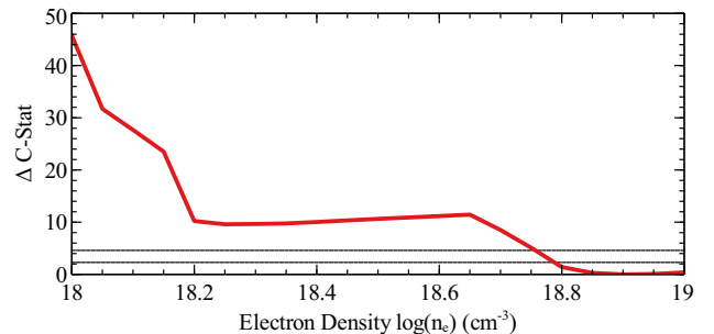
Figure 11. \Delta C -stat versus electron density value in logarithmic units. The two horizontal dotted and dashed lines are 1\sigma and 2\sigma measurement lines.
