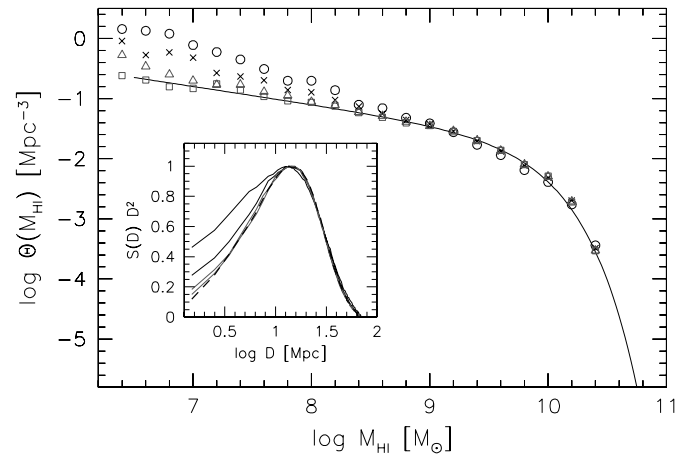
FIG. 6.—The Eddington effect. The solid line shows the HIMF of simulated data sets with a low-mass slope of \alpha = -1.3 . The symbols show the recovered 2DSWML HIMFs after Gaussian noise is added to the recession velocities of the galaxies: dispersion of 50 \text{ km s}^{-1} ( squares ), 100 \text{ km s}^{-1} ( triangles ), 200 \text{ km s}^{-1} ( crosses ), and 400 \text{ km s}^{-1} ( circles ).
