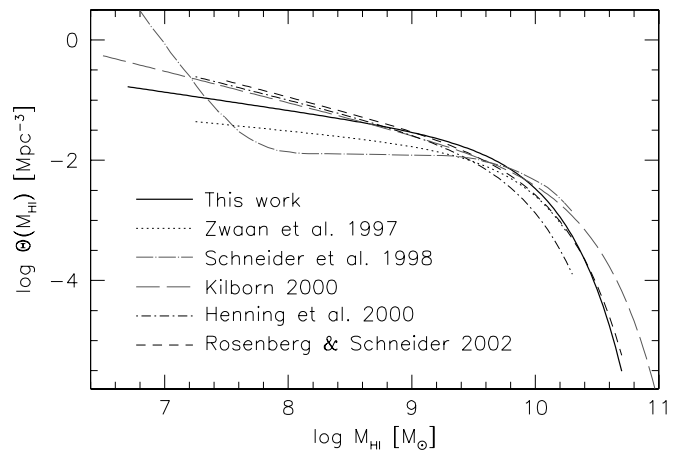
FIG. 12.—Comparison of the HIPASS BGC HIMF with previous calculations from blind H I surveys. Shown are HIMFs from AHISS (Zwaan et al. 1997), AS (Schneider et al. 1998), the HIPASS SCC (Kilborn 2000), the HIPASS HIZSS (Henning et al. 2000), and ADBS (Rosenberg & Schneider 2002). All mass functions have been converted to the same value of H_0 = 75 \text{ km s}^{-1} \text{ Mpc}^{-1} and are only plotted over the H I mass range in which they have been measured.
