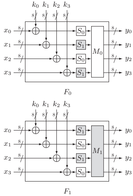
Fig. 3. F -functions
