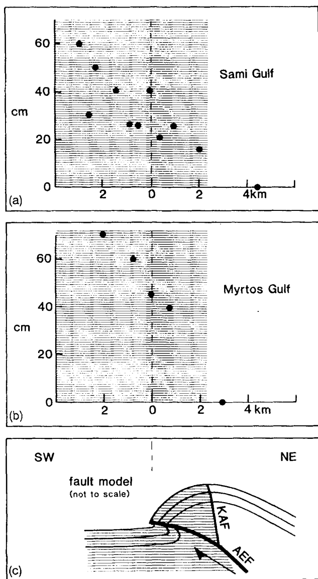
Figure 13. Uplift observed along the Sami Gulf (a) and Myrtos Gulf (b) versus distance from the surface trace of Aya Ephemia Fault (AEF). Values projected along axis B-B' in Fig. 9. The geometry (after Sorel 1976, modified) and the suggested direction of movement of AEF is shown in (c). The uplifted area is shaded and extends up to the Kalon Anticline Fault (KAF). Compare with Fig. 5.
