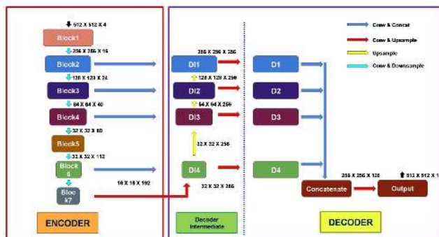
Figure 7: Team TeamTiger: proposed encoder-decoder architecture.
