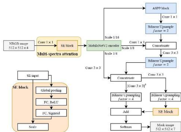
Figure 6: Team CNUPR_TH2L: pipeline.
