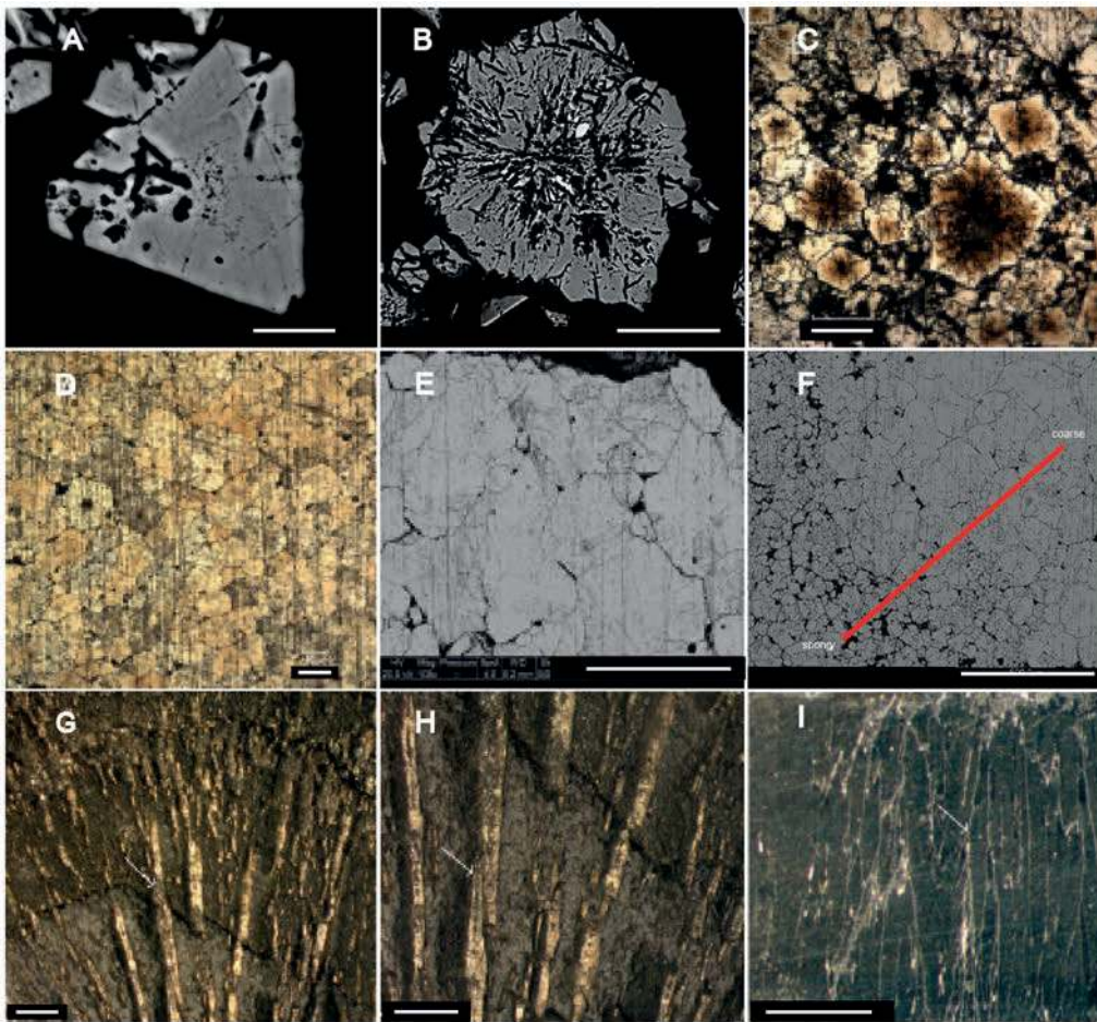
Figure 10. Petrography of pyrite crystals. (A) SEM-BSE image of an euhedral crystal after severe \text{HNO}_3 etching. Note the spongy texture in the centre and the growth bands in the outer part. (B) SEM-BSE image of floriform pyrite after severe \text{HNO}_3 etching. Note the radiating texture in the centre and the growth bands in the outer part. (C) Photomicrograph of the spongy pyrite after severe \text{HNO}_3 etching. This pyrite contains both euhedral and floriform pyrites. Note the orange colour in the centre of euhedral and floriform pyrites. (D) Photomicrograph of coarse pyrite after severe \text{HNO}_3 etching. Note small orange forms in the middle of some crystals. (E) SEM-BSE image of coarse pyrite after severe \text{HNO}_3 etching. (F) SEM-BSE view of the transition from spongy (lower left corner) to coarse (upper right corner) pyrite. (G–I) Pyrite “sun” sample (SMNH X4450) under reflected, plane-polarized light, highlighting the growth texture of pyrite. (G, H) Surface of the pyrite “sun” showing apparent growth bands (underlined in red) and elongated radiating crystals (arrow) centrifugally developed perpendicular to the growth bands. (H) Close-up view of G showing the relationships between radial crystals (arrow) and apparent growth bands. (I) Section parallel to the plane of the pyrite “sun” showing a centrifugal arrangement of coarse acicular crystals (arrow). Scale bars 10 \mu\text{m} (A), 50 \mu\text{m} (B, C), 100 \mu\text{m} (D, I), 500 \mu\text{m} (E, F), and 5 mm (G, H). doi:10.1371/journal.pone.0099438.g010
