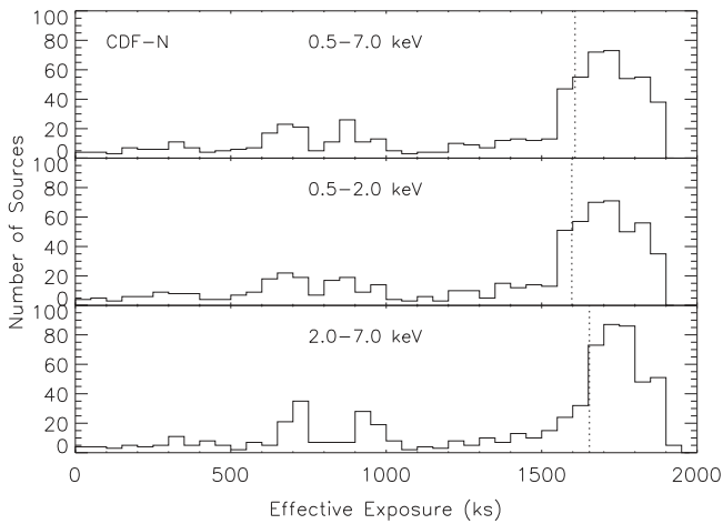
Figure 11. Distributions of effective exposure times for all the 683 2 Ms CDF-N main-catalog sources in the full, soft, and hard bands. The vertical dotted lines indicate the median effective exposures of 1607.5, 1597.0, and 1653.6 ks, for the full, soft, and hard bands, respectively.
