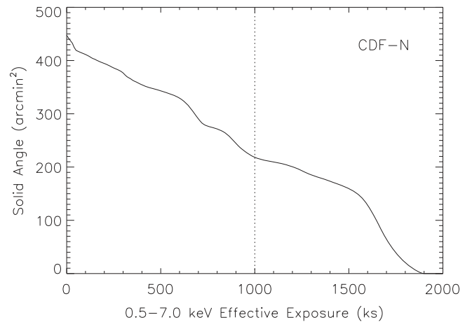
Figure 4. Survey solid angle as a function of minimum full band (0.5–7.0 keV) effective exposure for the 2 Ms CDF-N. The 2 Ms CDF-N covers a total area of 447.5 \text{ arcmin}^2 and has a maximum exposure of 1.896 Ms. The vertical dotted line denotes an effective exposure of 1 Ms. 218.3 \text{ arcmin}^2 (48.8%) of the CDF-N survey area has >1 Ms effective exposure.
