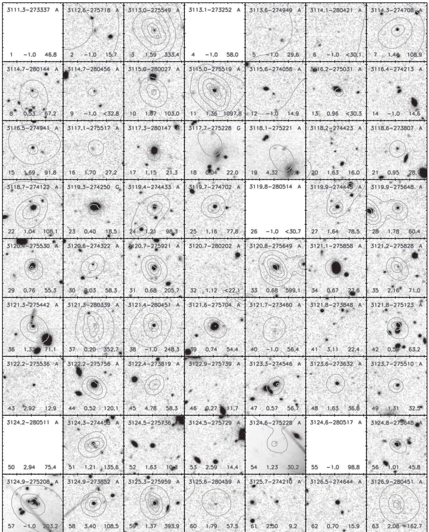
Figure 43. Same as Figure 42, but for the TENS WIRCam K_s band (Hsieh et al. 2012). In some cases there is no K_s -band coverage (e.g., XIDs = 1, 4, 26, 50, 55). (An extended version of this figure is available.)
