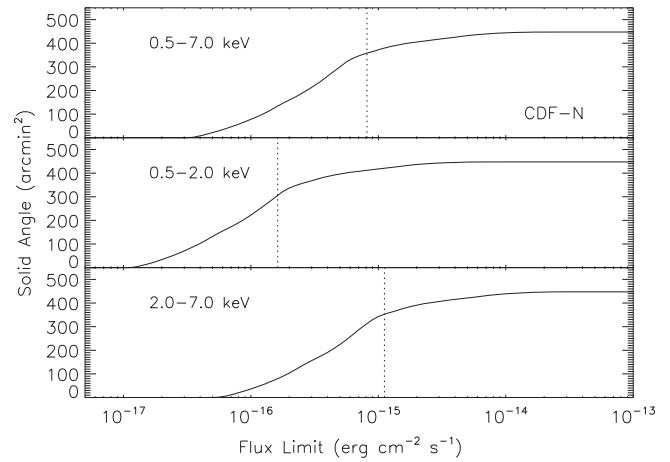
Figure 29. Survey solid angle as a function of flux limit in the full, soft, and hard bands for the 2 Ms CDF-N main catalog. The vertical dotted lines indicate the median fluxes of the main-catalog sources detected in the three bands.
