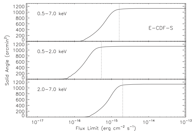
Figure 57. Survey solid angle as a function of flux limit in the full, soft, and hard bands for the 250 ks E-CDF-S main catalog. The vertical dotted lines indicate the median fluxes of the main-catalog sources detected in the three bands.
