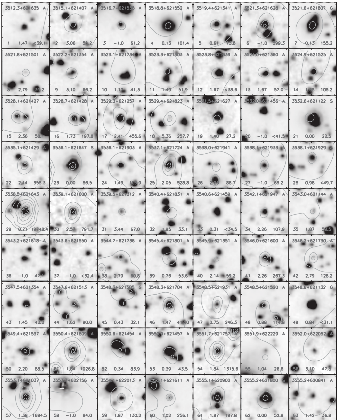
Figure 16. Same as Figure 14, but for the SEDS IRAC 3.6 \mu\text{m} band (Ashby et al. 2013). (An extended version of this figure is available.)
