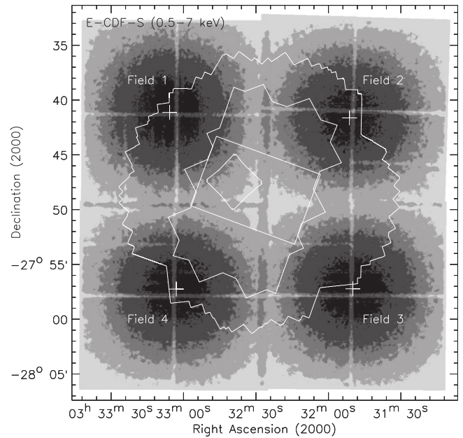
Figure 56. Full-band (0.5–7.0 keV) sensitivity map for the 250 ks E-CDF-S main catalog. The grayscale levels, ranging from black to light gray, denote areas with flux limits of <2.0 \times 10^{-16} , 2.0 \times 10^{-16} to 4.0 \times 10^{-16} , 4.0 \times 10^{-16} to 6.0 \times 10^{-16} , 6.0 \times 10^{-16} to 10^{-15} , and >10^{-15} erg cm -2 s -1 , respectively. The regions and the plus signs have the same meanings as those in Figure 30.
