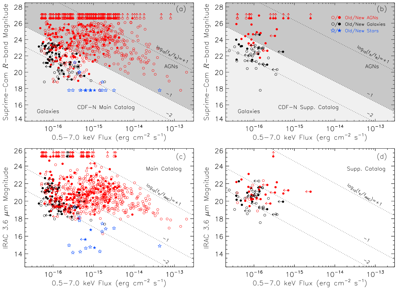
Figure 22. (Top) Suprime-Cam R -band magnitude vs. full-band flux for (a) the 2 Ms CDF-N main-catalog sources and (b) the supplementary-catalog sources. (Bottom) IRAC 3.6 \mu\text{m} magnitude vs. full-band flux for (c) the 2 Ms CDF-N main-catalog sources and (d) the supplementary-catalog sources. The meanings of the symbols of different types and colors are indicated by the legend. Arrows denote limits. In panels (a) and (b), diagonal dotted lines indicate constant full-band-to- R flux ratios, and shaded areas represent approximate flux ratios for AGNs (dark gray) and galaxies (light gray). In panels (c) and (d), diagonal dotted lines indicate constant full-band-to-IRAC- 3.6 \mu\text{m} flux ratios. Note that the stars lined up at R = 17.8 mag have their R -band magnitudes set to this value for plotting purposes as they are assigned negative magnitudes in the R -band catalog due to saturation ( R = 17.8 is one magnitude brighter than the brightest non-saturated stars in the R -band catalog).
