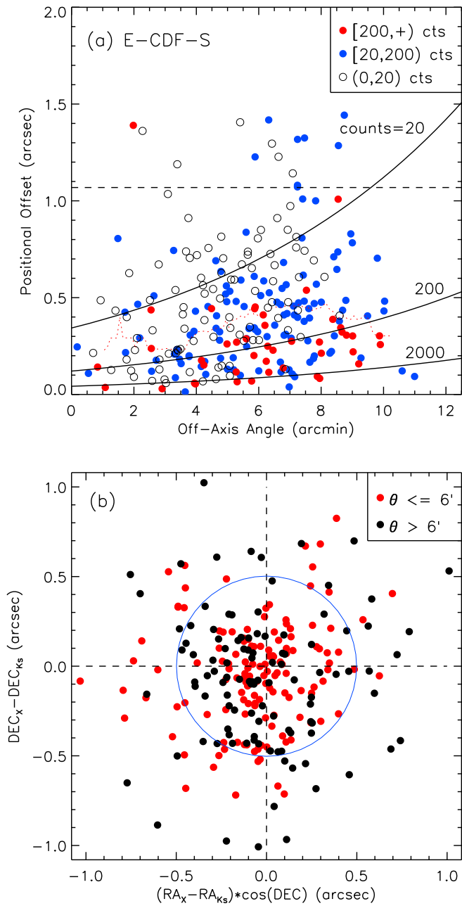
Figure 35. (a) Positional offset vs. off-axis angle for the 257 250 ks E-CDF-S main-catalog sources that have K_s \leq 20.0 mag counterparts in the TENIS WIRCam K_s -band catalog (Hsieh et al. 2012) utilizing a matching radius of 1''.5 (see Section 3.3.2 for the description of an apparent outlier, i.e., the red filled circle located at the top left corner, that deviates significantly from the relation defined as Equation (2)). Red filled, blue filled, and black open circles indicate X-ray sources with \geq 200 , \geq 20 , and < 20 counts in the energy band that is used to determine the source position, respectively. The red dotted curve denotes the running median of positional offset in bins of 2' . The horizontal dashed line represents the median offset ( 1''.07 ) of the false matches expected. The three solid curves correspond to the \approx 68\% confidence-level X-ray positional uncertainties (derived according to Equation (2)) for sources with 20, 200, and 2000 counts. (b) Positional residuals between the X-ray and K_s -band positions for the remaining 256 X-ray- K_s -band matches. Red and black filled circles represent sources with an off-axis angle of \leq 6' and > 6' , respectively. A blue circle with a 0''.5 radius is drawn at the center as a visual guide.
