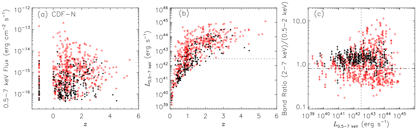
Figure 18. (a) Observed-frame full-band flux vs. adopted redshift, (b) absorption-corrected, rest-frame 0.5–7 keV luminosity vs. adopted redshift, and (c) band ratio vs. absorption-corrected, rest-frame 0.5–7 keV luminosity for the 2 Ms CDF-N main-catalog sources. Red open circles indicate old sources while black filled circles indicate new sources. Arrows denote limits. In panel (b), sources having no redshift estimates are not plotted; in panel (c), sources having no redshift estimates or sources having only full-band detections are not plotted. The dotted lines in panels (b) and (c) and the dashed–dotted line in panel (c) correspond to the threshold values of two AGN-identification criteria, L_{0.5-7 \text{ keV}} \geq 3 \times 10^{42} \text{ erg s}^{-1} and \Gamma \leq 1.0 .
