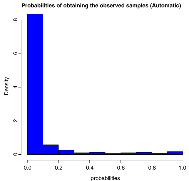
FIG. 4. Histogram of the probabilities of obtaining the samples observed in the exit polls using the official results as the probabilities of a Yes vote.
