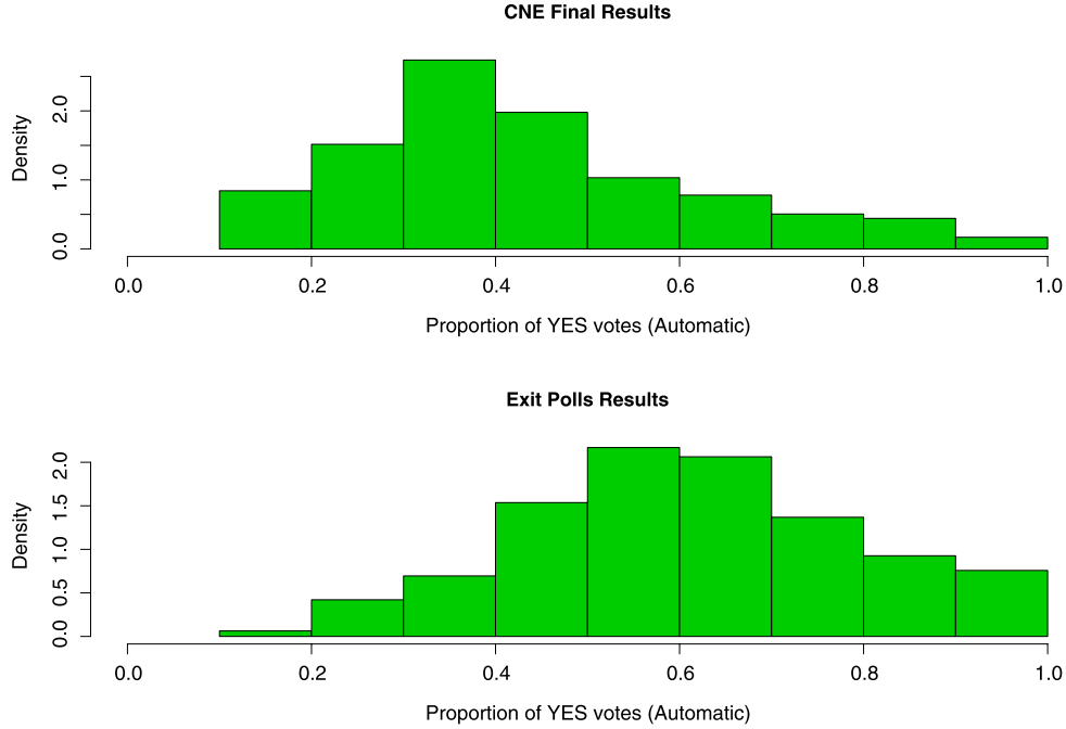
FIG. 3. Distribution of Yes vote proportions by center: official results (top panel), exit poll results (bottom panel).
