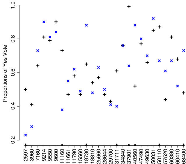
FIG. 1. Comparison of the common exit polls. The results from the SÚmate exit poll (indicated by +) and the PJ exit poll (indicated by x) are shown. Centers in which the two polls differ significantly are highlighted in the bottom margin. Significance is established at the 1% level. Numbers in the x axis correspond to the CNE coding of the centers.
