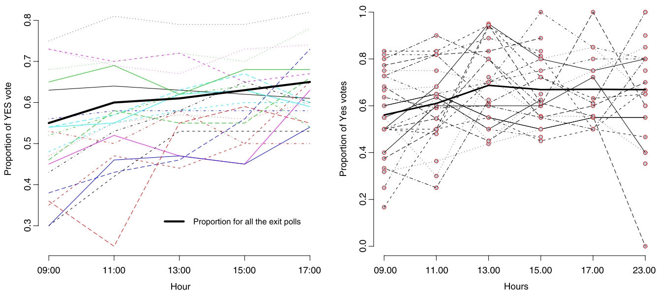
FIG. 2. Proportion of Yes votes at reporting times for the SÚmate exit poll: proportions for the states (left panel), proportions for the centers that were polled until 23:00 (right panel).
