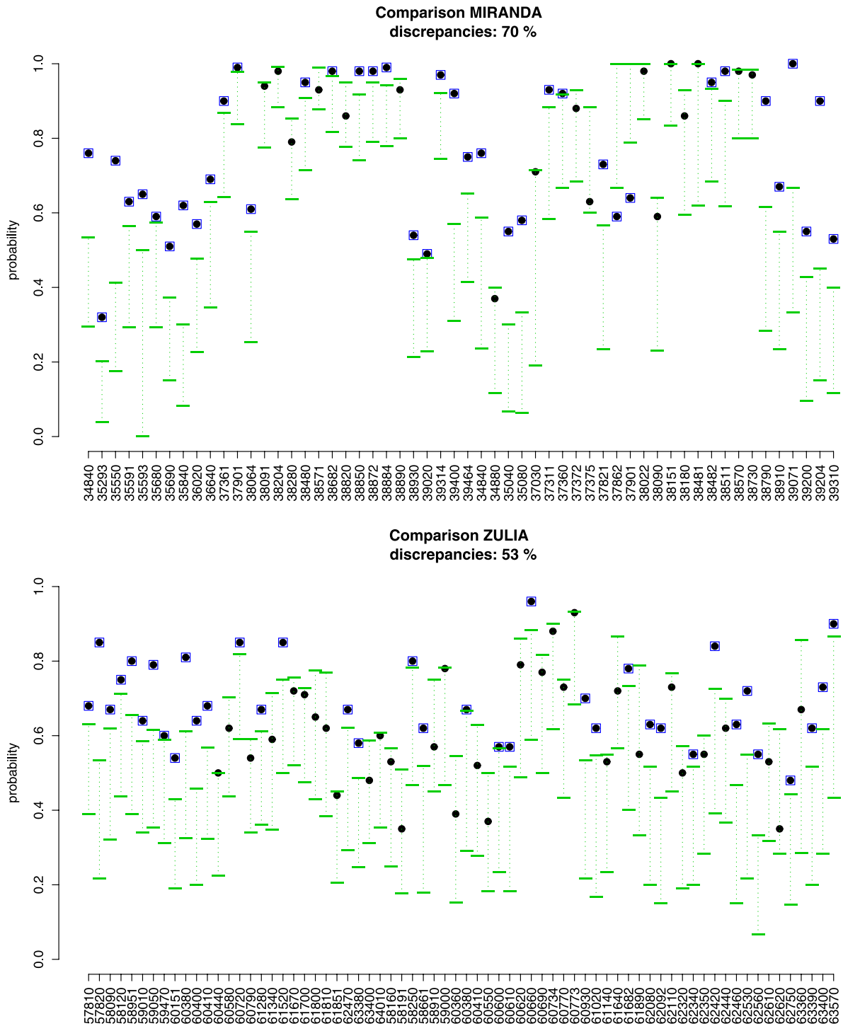
FIG. 6. 99% intervals for the proportions of Yes votes computed using 5000 simulated samples for each automatic center. The simulated samples were of the same size as the samples in the exit polls. The probability of a Yes vote was taken as the official one. The dotted lines denote the intervals. The exit poll results are marked with squares when they fall outside the corresponding intervals.
