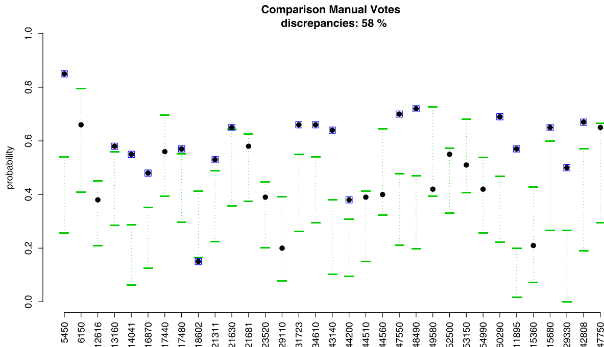
FIG. 7. 99% probability intervals for the proportions of Yes votes computed using 5000 simulated samples for each manual center. The simulated samples were of the same size as the samples in the exit polls. The probability of a Yes vote for a given center is taken as the official proportion of a Yes vote in such center. The dotted lines denote the intervals. Exit poll results are marked with squares when they fall outside the intervals.
