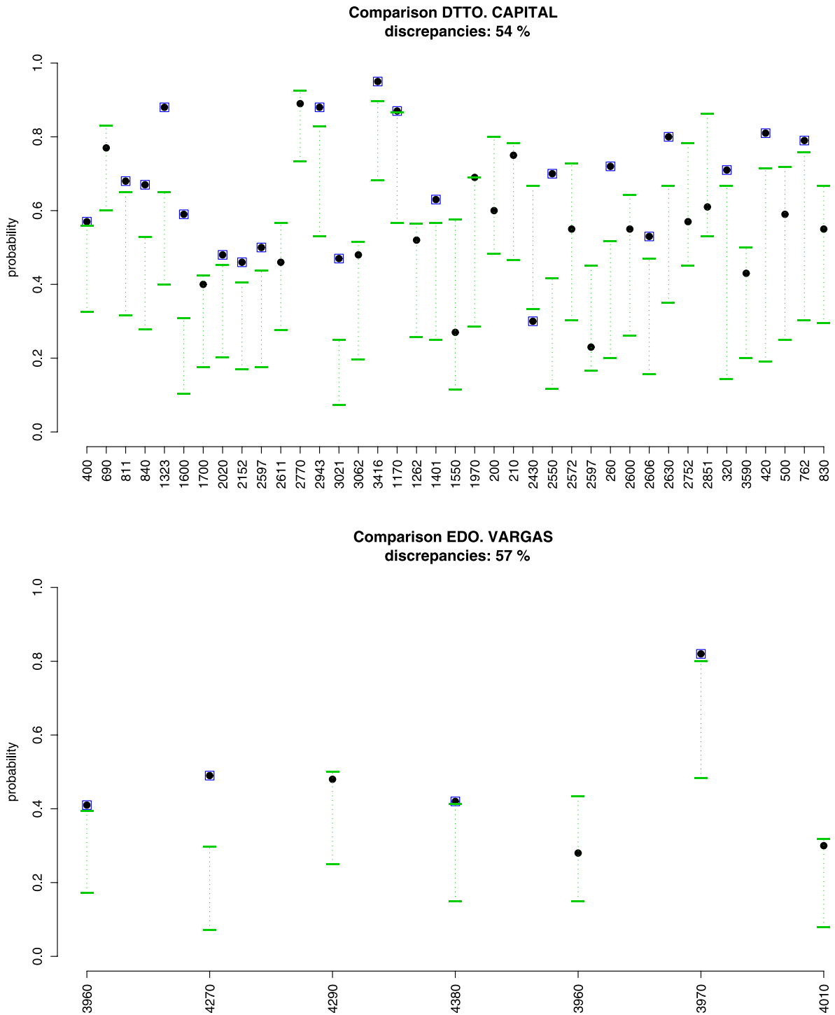
FIG. 5. 99% probability intervals for the proportions of Yes votes computed using 5000 simulated samples for each automatic center. The simulated samples were of the same size as the samples in the exit polls. The probability of a Yes vote was taken as the official one. The dotted lines indicate the intervals. The exit poll results are marked with squares when they fall outside the corresponding intervals.
