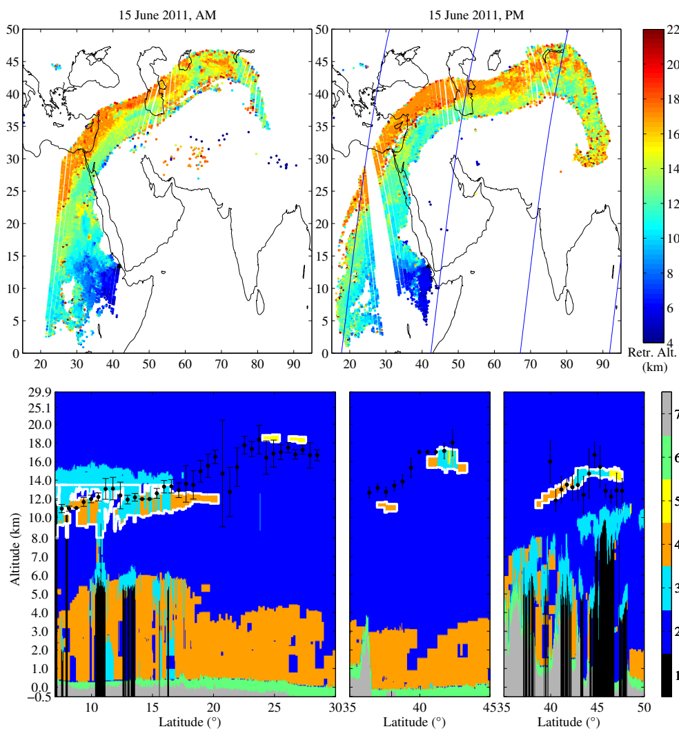
Fig. 6. IASI SO 2 height retrievals are presented on top from 4 to 22 km; blue lines indicate CALIPSO ground tracks within 5 h of the plume. In the bottom panels, the CALIOP the Level 2 product, “Vertical Feature Mask” is shown for the CALIPSO curtains corresponding to the ground tracks shown above, from left to right. Colours are numbered 1 to 7 indicated in the colour bar and stand for: no signal (1), clean air (2), cloud (3), aerosol (4), stratospheric feature (5), surface (6) and subsurface (7). Features which are likely to correspond to sulfate aerosols originating from Nabro are contoured in white on the CALIOP maps. Coincident IASI altitude retrievals are superimposed on these CALIOP maps as black dots, with a standard deviation representing the spread in retrieved altitudes around the overpass.
