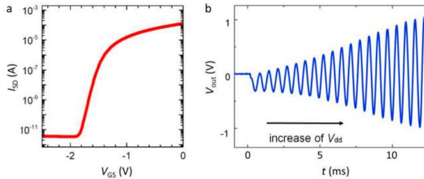
Figure 5. (a) Transfer curves of a LaAlO 3 -SrTiO 3 FET. The on/off ratio is six orders of magnitude and the subthreshold voltage swing is close to 60 mV dec -1 . (b) A monolithically integrated LaAlO 3 -SrTiO 3 ring oscillator. Upon increasing the supply voltage the output voltage oscillates with a RC time-constant-controlled oscillation frequency of 1.4 kHz. All data was measured at room temperature. Reprinted with permission from [74]. Copyright 2013 Wiley.
