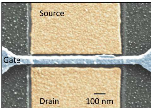
Figure 6. False-colour scanning electron microscopy image of a sub-100 nm gate length LaAlO 3 -SrTiO 3 transistor.
