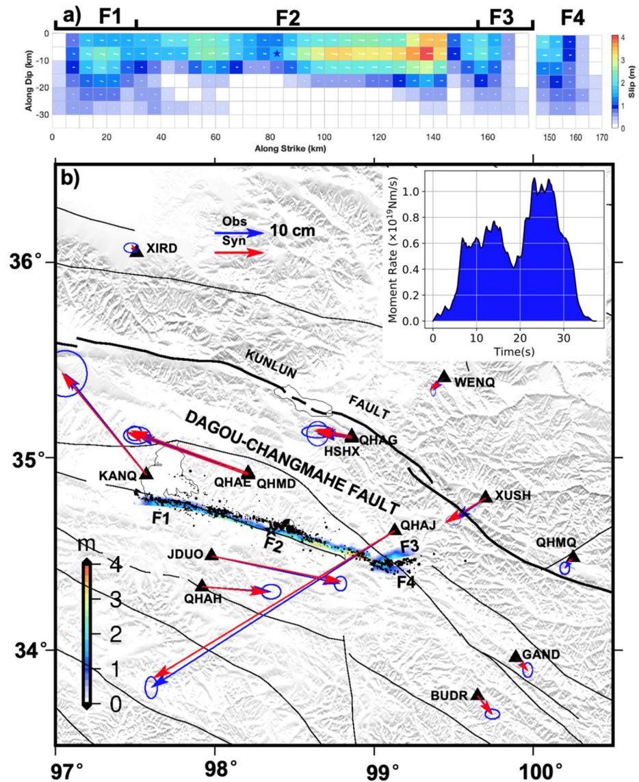
Figure 3. (a) Tile view of the final slip model. Blue star locates the epicenter and the arrows show the rake angle at each patch. (b) Comparison of measured (blue) and predicted (red) horizontal co-seismic displacements. Black dots show aftershocks determined by Wang et al. (2021). Color shading shows the best-fitting co-seismic slip distribution of the 2021 M_w 7.4 Madoi Earthquake from the joint inversion of all the data assembled in this study. Inset shows moment rate as a function of time.
