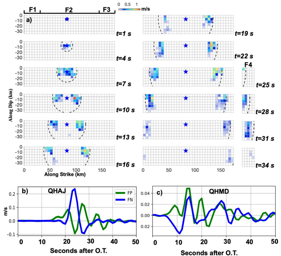
Figure 4. (a) Snapshots of the rupture evolution at 3 s time intervals. Black dashed line shows the isochron of rupture front for a rupture speed of 2.8 km/s (b) Fault-parallel and normal fault normal velocity at GNSS stations QHAJ and QHMD.
