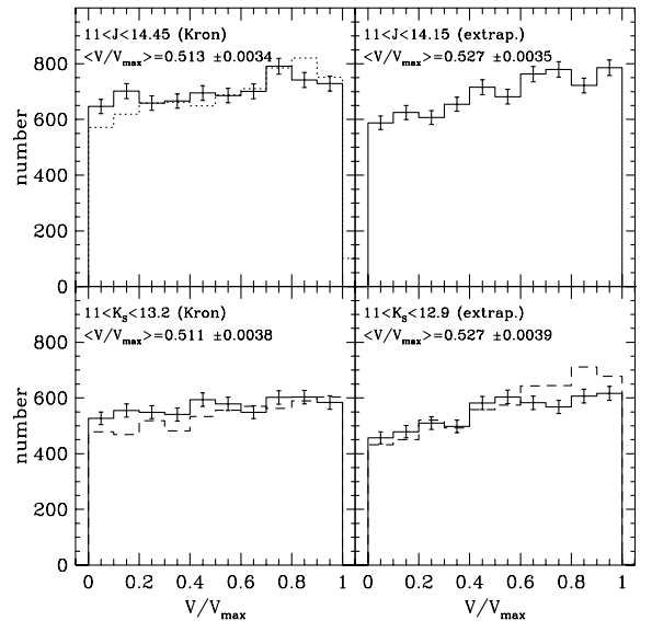
Figure 7. The distributions of V/V_{\text{max}} for our magnitude-limited samples. The solid histograms in the four panels show the V/V_{\text{max}} distributions for our J and K_S Kron and extrapolated magnitude-limited samples. The mean values of \langle V/V_{\text{max}} \rangle are indicated on each panel. The K_S -band magnitudes are those inferred from the J -band magnitudes and aperture colours. The distributions for the directly measured K_S -band Kron and extrapolated magnitudes are shown by the dashed histograms in the lower panels. The dotted histogram in the top-left panel shows the V/V_{\text{max}} distribution we obtain, when attempting to take account of the 2MASS isophotal diameter and isophotal magnitude limits in estimating the V_{\text{max}} values.
