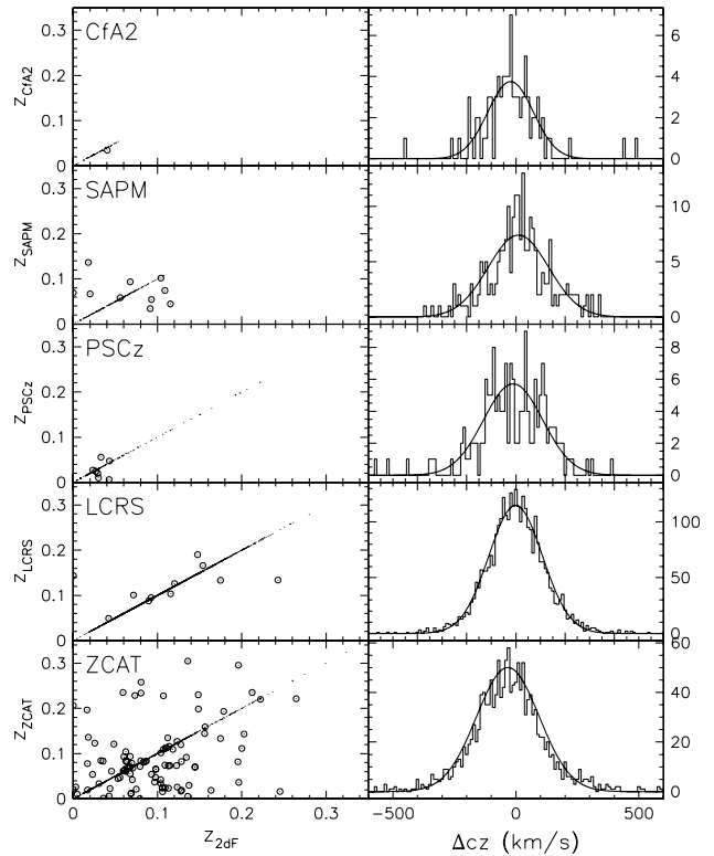
Figure 11. Comparisons of the 2dFGRS redshifts with those from the CfA2, SAPM, LCRS and ZCAT catalogues. The left-hand panels show the correlations between the redshift measurements, with each comparison shown as a dot. Most dots lie along the 1-to-1 line; the relatively few blunders ( |\Delta cz| > 600 \text{ km s}^{-1} ) are circled. The right-hand panels show the histogram of redshift differences overlaid with a Gaussian having the same median and rms.
