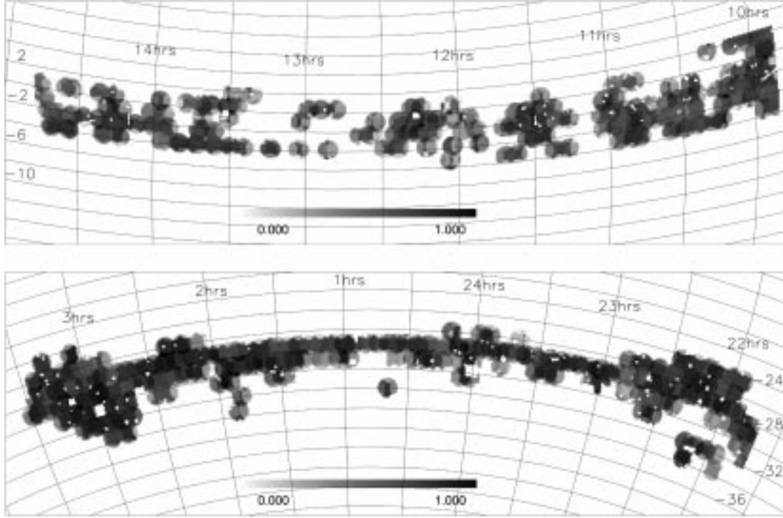
Figure 15. The redshift completeness, R(\theta) \equiv N_e(\theta)/N_p(\theta) as a function of position for the 100k public release dataset (2dFGRS data from 1997 October to 2000 January). The top panel is for the NGP, the bottom panel for the SGP, plotted in a zenithal equal-area projection.
