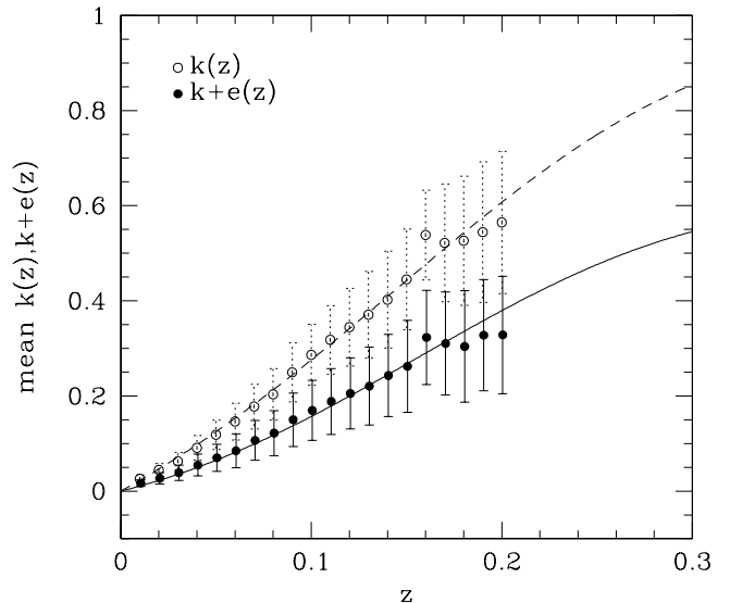
Figure 8. The curves show the fits, k(z) = (2.2z + 6z^2)/(1 + 15z^3) and k(z) + e(z) = (z + 6z^2)/(1 + 20z^3) , to the mean k , and k+e correction as a function of redshift. The mean corrections at each redshift, shown by the symbols, have been computed as a function of redshift from the known fractions of each spectral type. The error bars show the rms scatter about the mean of these distributions.
