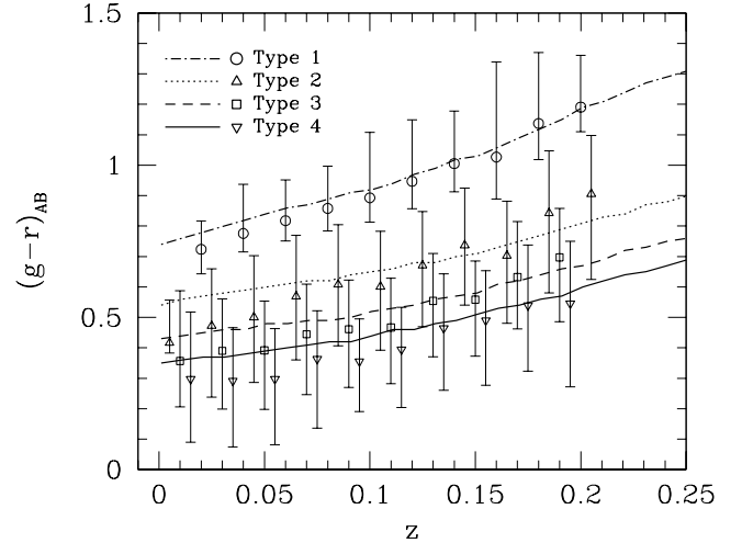
Figure 6. Galaxy g - r colours as a function of redshift. The symbols and error bars show, for each 2dFGRS spectral type, the median, 10 and 90 centiles of the g - r colour distribution, as a function of redshift. The curves are the predictions for model galaxies, computed using the Bruzual & Charlot stellar population synthesis code, the star formation histories of which have been selected to reproduce, as closely as possible, the median colour as a function of redshift in each class.
