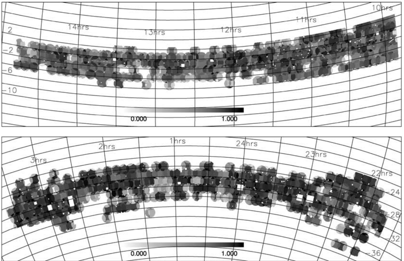
Figure 1. The sky coverage of the 2dFGRS data set analysed in this paper. This data set includes galaxy redshifts from all fields observed before 2001 May that have a redshift completeness greater than 70 per cent. As the fields overlap and many are still to be observed, the completeness varies across the sky. The quantity represented by the grey-scale is the sector redshift completeness, R(\theta) , defined in Appendix A.
