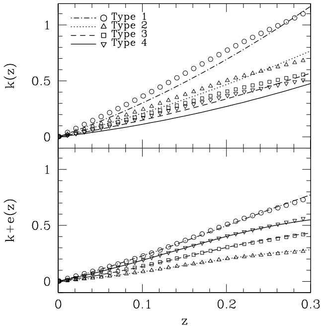
Figure 7. Model k and k+e corrections for each 2dFGRS spectral type. The symbols in the top panel show the k corrections for four models selected to match the g-r colours as a function of redshift plotted in Fig. 6. The curves show the corresponding k corrections adopted in Madgwick et al. (2002). The symbols in the lower panel show our model k+e corrections. In this case, the smooth curves are simple analytic fits [Type 1: k+e = (2z + 2.8z^2)/(1 + 3.8z^3) , Type 2: k+e = (0.6z + 2.8z^2)/(1 + 19.6z^3) , Type 3: k+e = (z + 3.6z^2)/(1 + 16.6z^3) , Type 4: k+e = (1.6z + 3.2z^2)/(1 + 14.6z^3) ].
