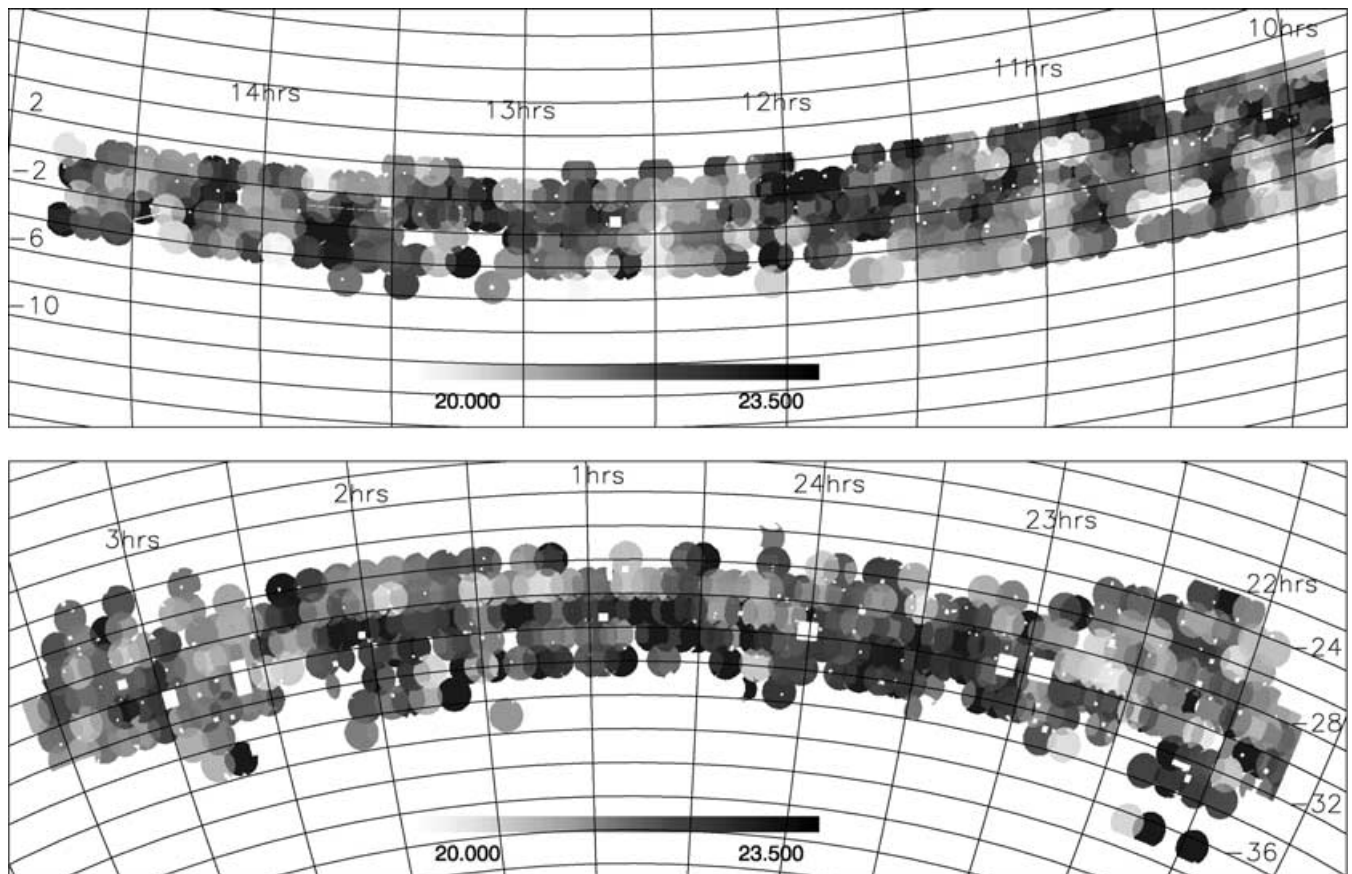
Figure A1. Map showing the variation of the parameter \mu with position on the sky. The dependence of the redshift completeness on apparent magnitude is accurately described by the fitting function c_2(b_J, \mu) = 0.99[1 - \exp(b_J - \mu)] .
