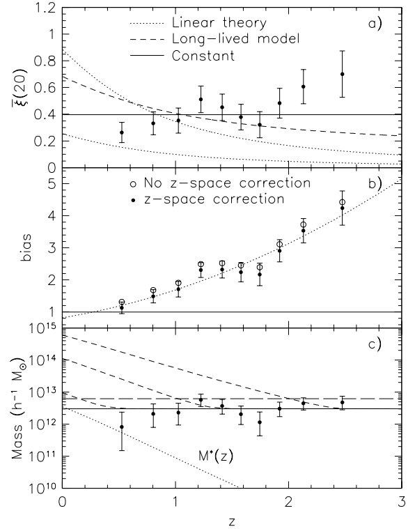
Figure 21. (a) Our measurement of \bar{\xi}(20) for 2QZ QSOs as a function of redshift (filled points). The data are compared to linear theory gravitational evolution (dotted lines) for two normalizations, one normalized to a WMAP /2dF cosmology (lower dotted line) and a second normalized to provide a ‘best fit’ to the data points (upper dotted line). We also compare to the best fit for a constant \bar{\xi}(20) (solid line) and a long-lived model (short dashed line). (b) The QSO bias, b_Q(z) , as a function of redshift derived from a comparison of \bar{\xi}(20) for QSOs to that expected for the WMAP /2dF cosmology. The open points are the raw bias values, i.e. \bar{\xi}_Q(s)/\bar{\xi}_p(r) , while the filled points with error bars are the values after making a consistent correction for z -space distortions. A simple empirical model is also shown (dotted line). (c) The mean mass of DMHs containing QSOs derived from the measured bias (filled points). We also show the mean mass averaged over redshift (solid line) and the mean plus twice the rms of the points (long dashed line). M^*(z) , the characteristic mass which is just collapsing at a given redshift, is denoted by a dotted line. The short dashed lines show the median expected growth in DMH mass from the mean DMH mass of QSO hosts at z = 0.53, 1.41 and 2.48 .
