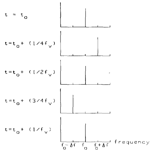
Fig. 2. Instantaneous "carrier" frequency for several instants during one cycle of vibration.
