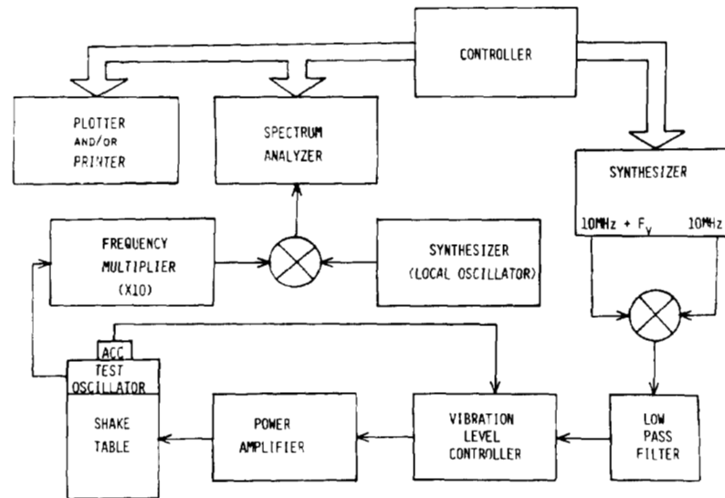
Fig. 7. Typical equipment configuration for measurement of acceleration-sensitivity using sinusoidal acceleration.
