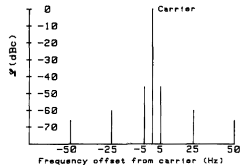
Fig. 4. Vibration-induced sidebands and carrier resulting from sinusoidal acceleration at 5 Hz, 25 Hz, and 50 Hz.
