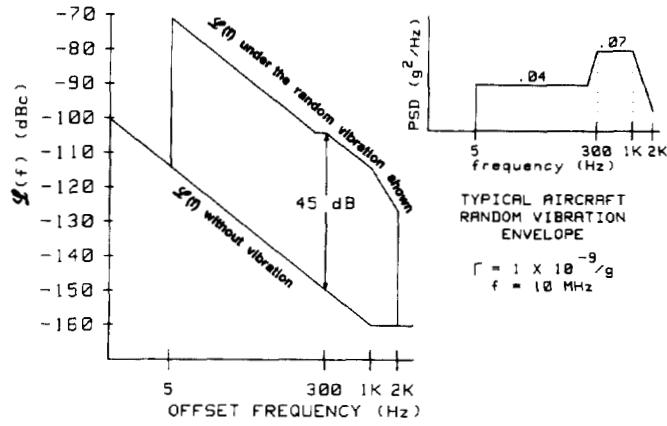
Fig. 6. Random vibration-induced phase noise and random vibration envelope.
