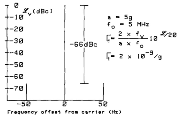
Fig. 8. Sample acceleration-sensitivity measurement using sinusoidal acceleration.
