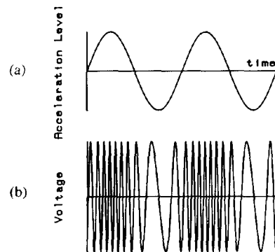
Fig. 3. (a) Acceleration level versus time. (b) Resulting oscillator output showing frequency modulation.
