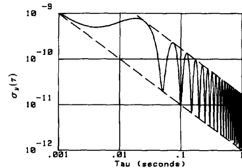
Fig. 5. Sigma of y of oscillator with acceleration-sensitivity of 1 ppb/g during 1-g vibration at 20 Hz.
