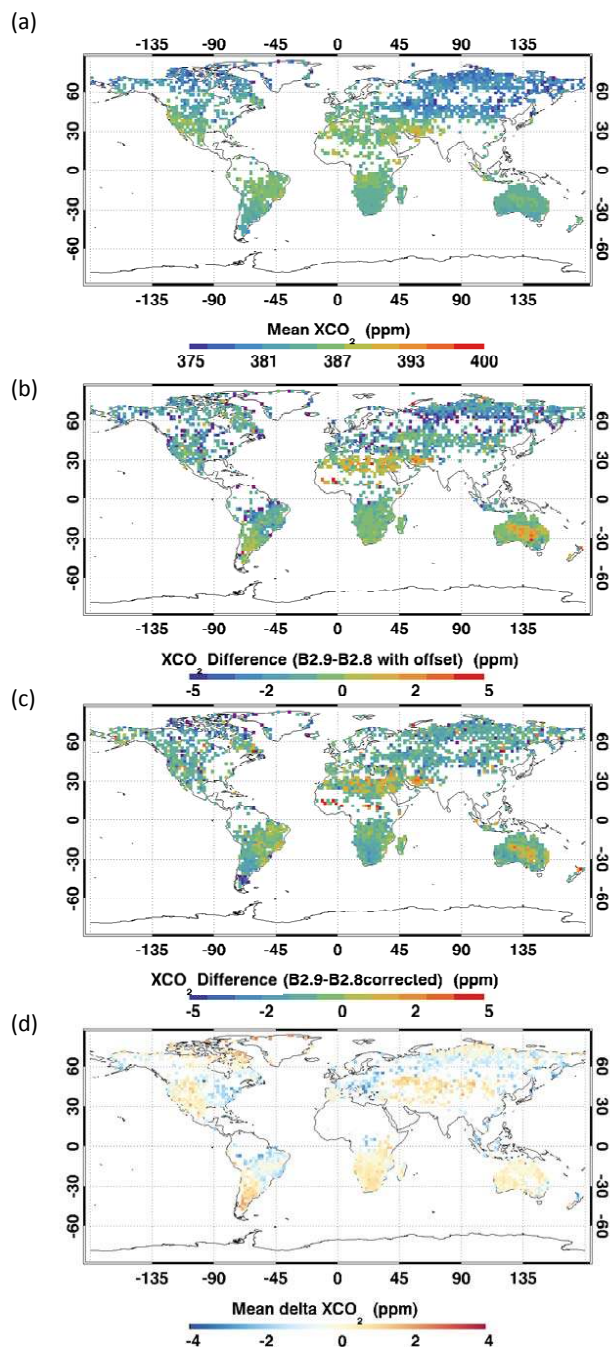
Fig. 17. Comparison of the preliminary B2.9 product with rescaled and corrected versions of the B2.8 product. (a) Map of the B2.9 product for July 2009, using the same post-processing filters used for the B2.8 results. (b) Difference between the B2.9 product and the B2.8 product, offset by ~7 ppm to remove the global X CO 2 bias. (c) Difference between the raw B2.9 product and the B2.8 results corrected for bias with the empirical approach developed by Wunch et al. (2011b). (d) Differences between the B2.9 results corrected for bias with the empirical approach developed by Wunch et al. (2011) and raw B2.9 product.
