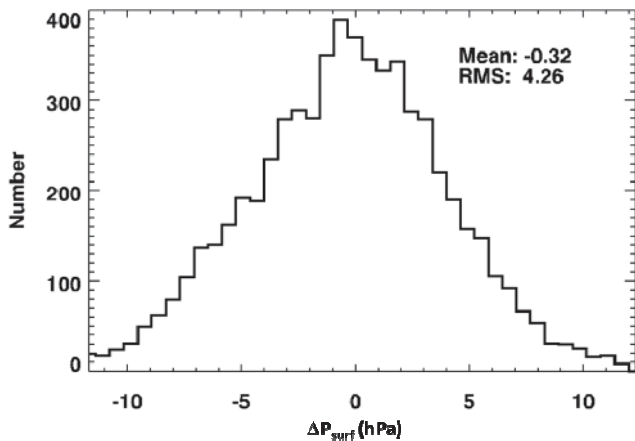
Fig. 14. Histogram of differences between the retrieved pressure and the ECMWF prior, \Delta P_{\text{surf}} for sounding retrieved using scaled ABO2 absorption coefficients. The data set used here includes all soundings over land collected in 23–25 April 2009, 1–31 July 2009; 18–20 September, and 14–16 January 2010 that pass the 85° solar zenith angle and cloud screening tests. Rescaling the O 2 absorption coefficients largely eliminates the global bias and yields a standard deviation comparable to that assumed in the a priori covariance matrix ( \pm 4 hPa).
