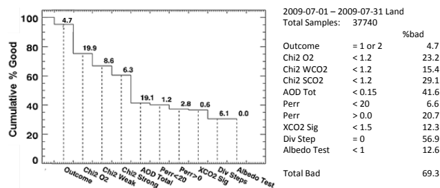
Fig. 10. Throughput of post-screening filters for July 2009. Histogram of reductions in the number of soundings by each step in the screening process (left) and the filter criterion and total fraction of the soundings that would be eliminated by each filter (right). The filters are applied from left to right, such that bad soundings are rejected by the first filter criterion that they fail. Chi2 O 2 , Chi2 Weak, and Chi2 Strong are the values of \chi^2 for the ABO 2 , SCO 2 and SCO 2 bands, respectively. AOD Total is the column integrated cloud and aerosol optical depth at 755 nm, Perr is the difference between the retrieved surface pressure and the ECMWF prior, X CO 2 Sig is the a posteriori CO 2 error, Div Steps is the number of diverging steps, and Albedo Test refers to the “blended albedo” filter introduced by Wunch et al. (2011), which rejects soundings over ice-covered surfaces where the albedo (and SNR) in the SCO 2 channel is much lower than that for the ABO 2 channel.
