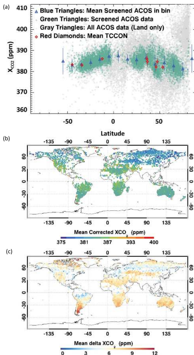
Fig. 13. ACOS GOSAT 2.8 retrievals from July 2009, corrected using the empirical regression formula developed by Wunch et al. (2011b). (a) Corrected B2.8 soundings that pass the nominal B2.8 screens (green triangles) and their averages in 10° zonal bins (blue triangles) are compared to TCCON measurements (red diamonds). (b) Spatial map of corrected B2.8 soundings. (c) Differences between the XCO 2 retrievals shown in Fig. 13b and the raw B2.8 retrievals shown in Fig. 1. After removing a ~7 ppm global offset, the empirical correction yields reduced XCO 2 over the tropics and northern mid-latitudes and higher values elsewhere. The combination of relatively large solar zenith angles and the presence of snow and ice cover in Patagonia contribute to the large positive air mass and blended albedo corrections there.
