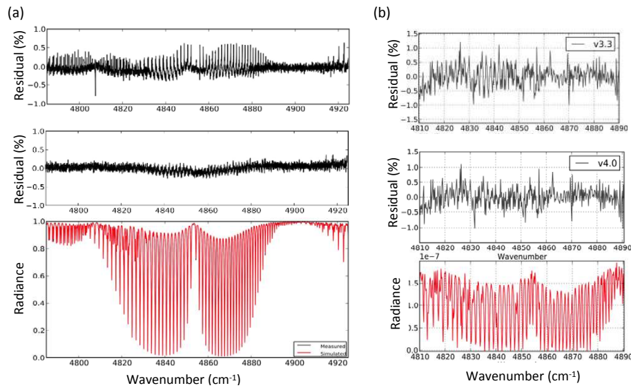
Fig. 5. (a) Spectral residuals in fits to laboratory spectra of the SCO 2 band (bottom) for the absorption coefficients used here (top), and values from the more recently implemented multi-spectral fitting approach (center). (b) Same as (a) for TANSO-FTS spectra collected in the vicinity of the Lamont Oklahoma TCCON station.
