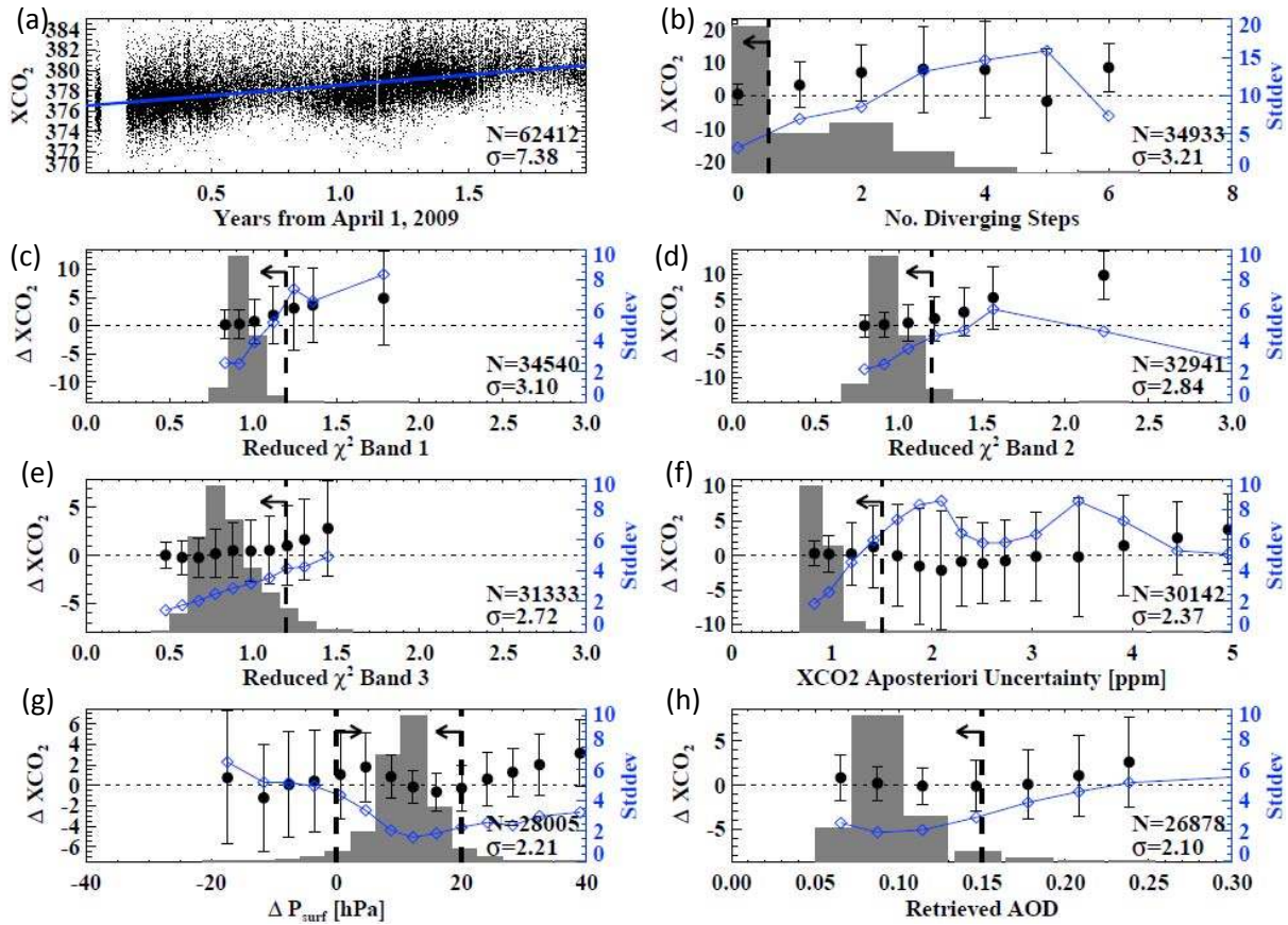
Fig. 8. Derivation of the post-processing filters applied to ACOS B2.8 data products. (a) X CO 2 estimates from all cloud-free soundings collected over land at latitudes between 20° S and 70° S between 4 April 2009 and 19 April 2011. The blue line indicates the secular trend in X CO 2 . Other panels show a histogram of the distribution of soundings as a function of the filtering variable (grey boxes) as well as: (i) the difference between the ACOS GOSAT X CO 2 estimates and a spatially-invariant X CO 2 background derived from TCCON data collected at latitudes between 20° S and 70° S, \Delta X_{CO_2} , (black points with 1- \sigma error bars) for each bin in the histogram; (ii) the standard deviation in \Delta X_{CO_2} for each bin in the histogram (blue diamonds and blue line, quantified as Stddev on the right-hand ordinate), and (iii) the range of values that pass the filter (dashed vertical lines with horizontal arrows). The number of points that passes the each filter, N, and the standard deviation in \Delta X_{CO_2} for this ensemble, \sigma , are shown in the lower right of each panel. The filtering variables include the number of diverging steps in the retrieval (b), the reduced \chi^2 for the fit in the 3 SWIR bands (c–e), the X CO 2 a posteriori uncertainty (f), the difference between the retrieved and a priori (ECMWF) surface pressure, \Delta P_{surf} (g), and the total aerosol optical depth at 0.755 \mu\text{m} , AOD. The panels are shown with the cumulative effect of each previous filter applied, so that only soundings passing all previous filters are used in any given panel.
