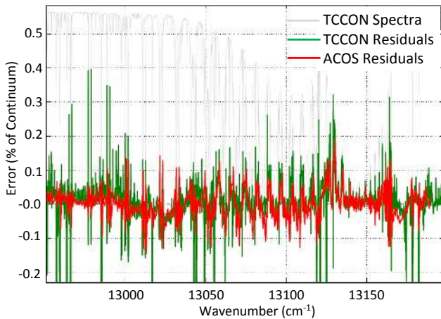
Fig. 6. Comparison of spectral residuals in the O 2 A-band from TCCON (green) and ACOS GOSAT (red) retrievals, along with a TCCON O 2 A-band spectrum (light grey).
