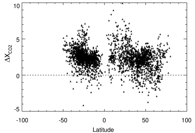
Fig. 15. Increase in X CO 2 produced by correcting the ILS interpolation error recently identified in the B2.8.
