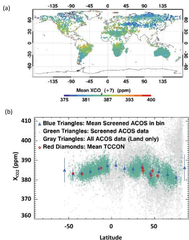
Fig. 12. (a) Map of all ACOS GOSAT B2.8 XCO 2 soundings over land for July 2009 that passed all pre- and post-screening filters. (b) The ACOS GOSAT B2.8 XCO 2 estimates shown in Fig. 1 have been divided by 0.982 to remove the global component of the bias and improve their agreement with contemporaneous TCCON retrievals.
