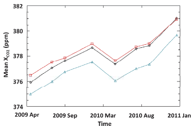
Fig. 3. Mean X CO 2 estimates over Australia are shown as a function of time for three different estimates of the time-dependent throughput of the TANSO-FTS. The blue curve shows X CO 2 retrievals assuming that the radiometric calibration coefficients derived from pre-launch tests did not change. A preliminary version of the time-dependent throughput correction was included in the B2.8 product (black line). A refined, time-dependent throughput correction that was developed more recently (red curve), produces an additional X CO 2 correction that decreases from ~0.5 ppm early in the GOSAT mission to slightly less than zero in early 2011.
