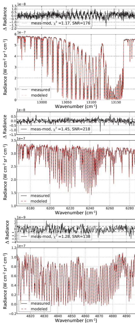
Fig. 4. Synthetic (red) and measured (black) spectra for a converged retrieval of a sounding acquired at 41.2° N, –95.8° E on 22 July 2010, just north of the Lamont Oklahoma TCCON station. This was a relatively bright sounding, collected at a solar zenith angle of 25.2° and an observation zenith 20.8°, yielding signal to noise ratios of 176, 218, and 138 in the ABO 2 , WCO 2 , and SCO 2 bands, respectively. The retrieved X CO 2 , surface pressure, and aerosol optical depth at 0.755 μm for this sounding were 388.7 ppm, 975.8 hPa, and 0.11, respectively.
