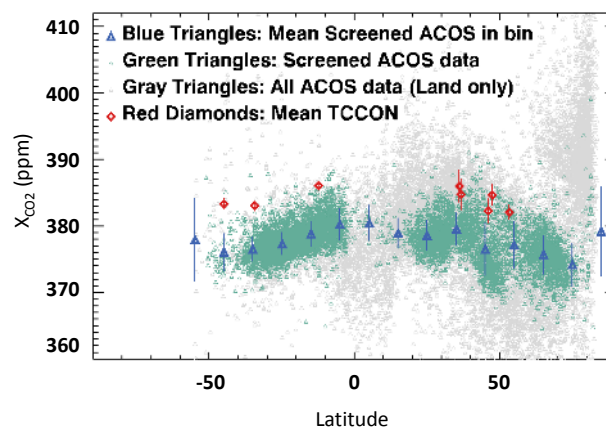
Fig. 1. All converged, cloud-free ACOS GOSAT B2.8 X CO 2 retrievals for soundings acquired over land at solar zenith angles <85° during July 2009 (grey triangles) are compared to TCCON retrievals from that month (red diamonds). ACOS GOSAT soundings that also pass a series of post-processing filters (see text) are over-plotted as green triangles. These screened values have been averaged over 10° wide zonal bands to derive the zonal mean estimates of X CO 2 (blue triangles with 1-σ error bars). The TCCON results are from the stations listed in Table 2.
