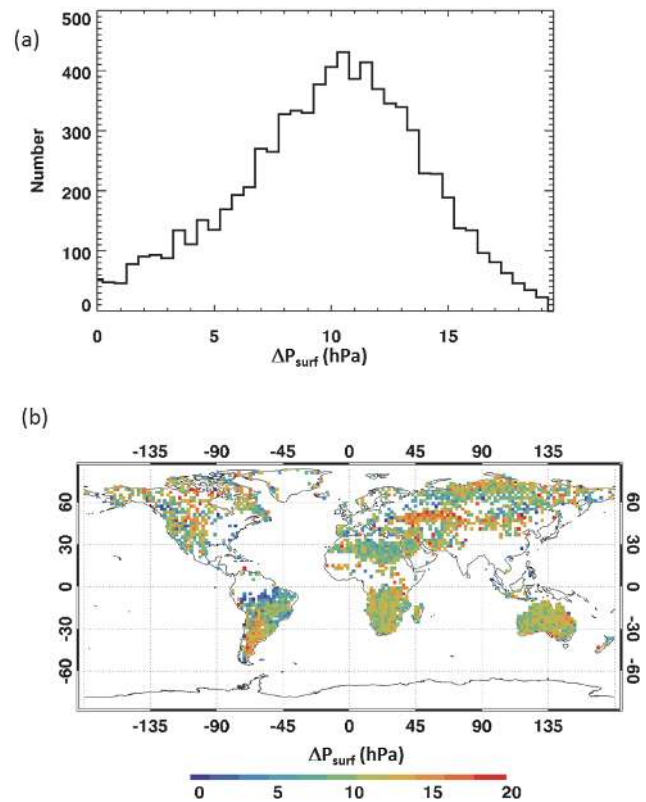
Fig. 2. (a) Histogram of differences between the retrieved surface pressures and the surface pressure prior estimated from ECMWF data, \Delta P_{\text{surf}} (hPa), for all soundings over land in July 2009. (b) Map of differences between the retrieved surface pressure and the prior for July 2009.
