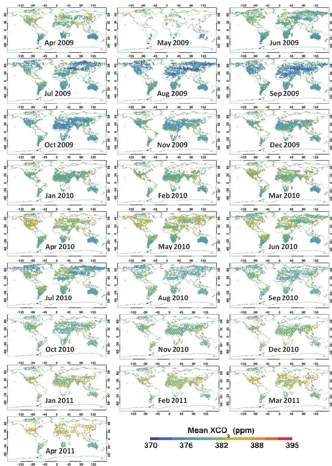
Fig. 11. ACOS GOSAT B2.8 X CO 2 retrievals for April 2009–April 2011. Each map shows the X CO 2 values retrieved over a 1-month interval. Each symbol indicates the average of all X CO 2 estimates in a 2 \times 2^\circ bin for that month that passed all pre- and post-screening filters. The coverage in May 2009 is limited because TANSO-FTS was still being commissioned and few soundings were collected. The data used to create the maps can be obtained from the NASA GES DISC.
