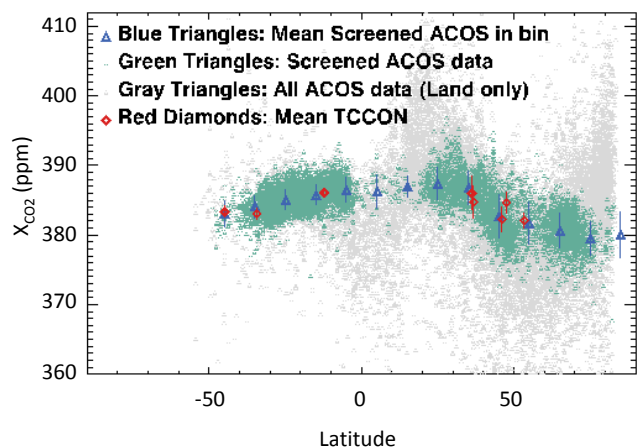
Fig. 16. Same as Fig. 1, but for ACOS GOSAT B2.9. This version of the algorithm incorporates scaled O 2 A-band absorption cross-sections, improved WCO 2 cross-sections, corrected ILS interpolation, a zero-level-offset retrieval, and other improvements to yield a much better fit to the TCCON results at all latitudes.
