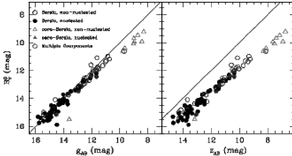
FIG. 16.— Comparison of the g and z -band total magnitudes, corrected for extinction, derived by integrating to infinity the best fitting surface brightness profiles, compared to the B_{g0}^0 magnitudes from the RC3. The diagonal line shows a one-to-one correspondence. Galaxies with multiple morphological components, for which the model fits are not always satisfactory, are plotted in blue.
