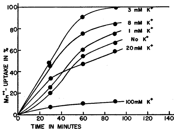
FIG. 4. The influence of K^+ concentration on the absorption of Mn^{++} by respiring yeast. The yeast concentration was 100 mg./ml.; phosphate, 7.5 \times 10^{-4} M; Mn^{++} , 7.5 \times 10^{-4} M; and glucose, 0.1 M. Corrections were made for surface binding, by controls with no glucose.
