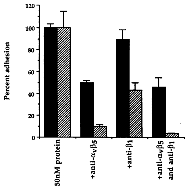
Figure 7. The \beta_1 integrin on smooth muscle cells acts as an osteopontin not a vitronectin receptor. Wells were precoated with 50 nM solutions of either vitronectin (3.5 \mu\text{g}/\text{ml} , solid bars) or osteopontin (3.25 \mu\text{g}/\text{ml} , hatched bars). \alpha_v\beta_3^- cells were plated in the absence (no antibody) or presence of a 1:500 dilution of ascites of anti- \alpha_v\beta_5 (PIF6), anti- \beta_1 (P4C10), or both. Adhesion was quantitated after 60 min, and data are expressed as means \pm SEM.
