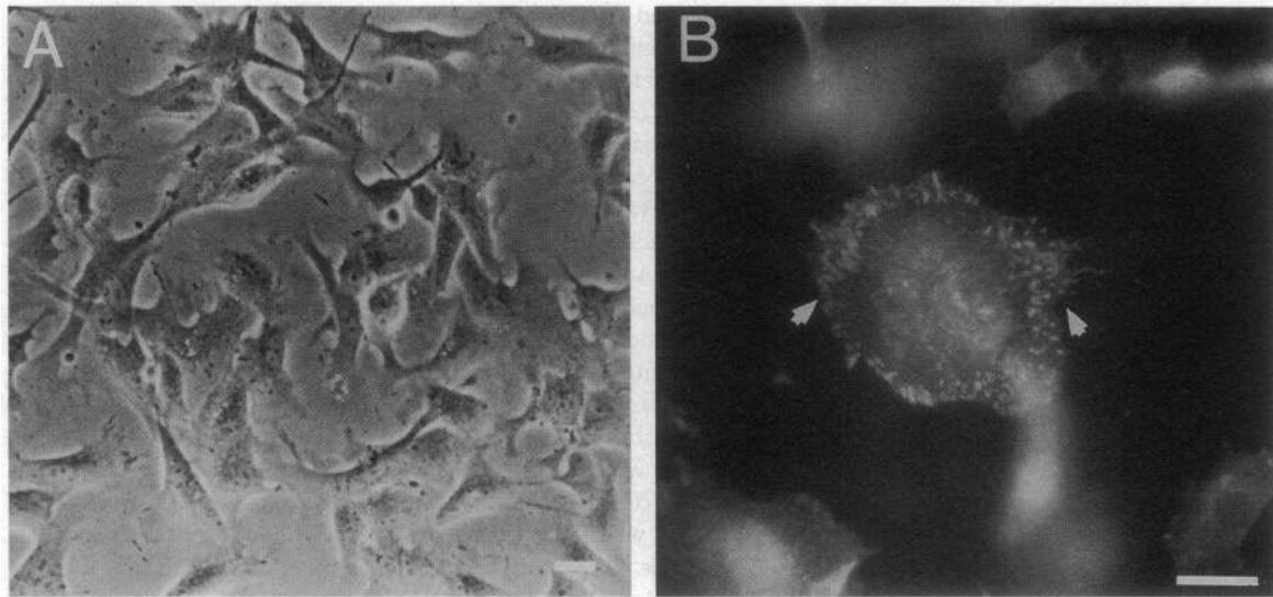
Figure 3. Adhesion of \alpha_v\beta_3^- cells on osteopontin is accompanied by cell spreading and focal contact formation. (A) \alpha_v\beta_3^- cells were plated in wells precoated with a 3.25- \mu\text{g/ml} solution of osteopontin and allowed to incubate for 60 min. The phase photograph was taken after nonadherent cells were washed off. Bar = 20 \mu\text{m} . (B) \alpha_v\beta_3^- cells were plated in wells precoated with a 3.25- \mu\text{g/ml} solution of osteopontin, rinsed, and fixed after 60 min. Cells were stained with antivinulin, followed by a fluorescein-conjugated rabbit anti-mouse IgG. Vinculin localizes to focal contacts (white arrows). Bar = 20 \mu\text{m} . Original magnification of A was 200 and B was 400.
