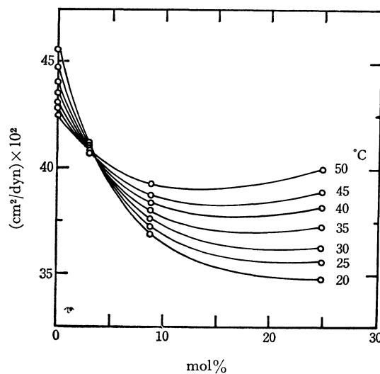
Fig. 12. Compressibility vs. concentration of DMF aqueous solutions.
