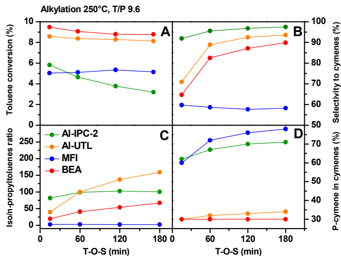
Fig. 19 Time-on-stream dependence of toluene conversion (A), selectivity to cymenes (B), iso/n -propyltoluenes ratio (C) and p -cymene selectivity (D) in toluene alkylation with isopropyl alcohol at 250 °C for four different zeolites; Al-IPC-2, Al-UTL, MFI and BEA.
