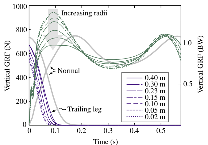
Fig. 4. Vertical ground reaction forces (GRF) versus time over one step, measured during walking with arcs of different radius and in normal shoes. Larger arc radii resulted in smoother collisions during the step-to-step transition. Small arc radii resulted in very large initial peaks in ground reaction force. With larger arcs this peak decreased to below its magnitude in normal walking, but it always occurred earlier in the step. Walking on arcs resulted in shorter double-support times, decreasing with smaller radii. Arc radius had little effect on the second peak in vertical force. Data shown are averaged over all subjects and plotted over the mean step period. A step begins at heelstrike and ends at opposite heelstrike, with double support occurring over the first 0.10–0.15 s. BW, body weight. Blue and green traces indicate forces under the trailing and leading legs, respectively.
