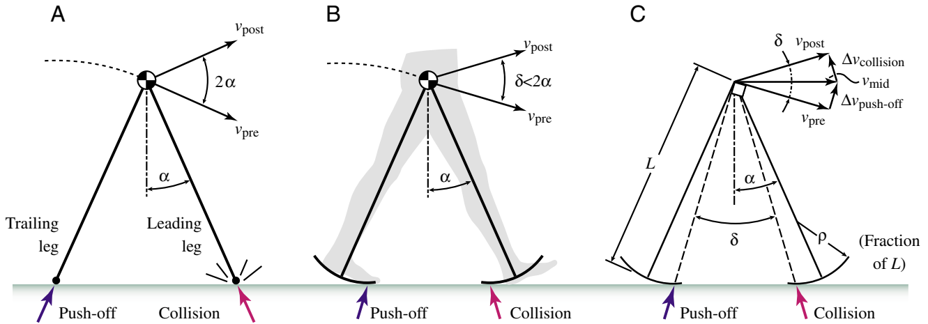
Fig. 1. A simple model demonstrates how a rolling foot can affect walking energetics. (A) Modeling the legs as pendulums supporting the body center of mass (COM), a step can be produced by passive limb dynamics with no energy input (McGeer, 1990a). Work is required, however, in the step-to-step transition to redirect the COM velocity. This can be accomplished with positive push-off work performed by the trailing leg, and negative collision work by the leading leg (Kuo, 2002). These leg actions redirect the pre-transition COM velocity v_{pre} to a post-transition velocity v_{post} . For point feet, the net directional change in velocity is equal to the angle between the legs, 2\alpha . (B) A model with arc feet applies collision at the heel of the leading leg, and push-off at the toe of the trailing leg. This reduces the directional change \delta in COM velocity and therefore the step-to-step transition work. (C) COM velocity change may be understood geometrically. The pre-transition velocity v_{pre} is directed perpendicular to the line from the trailing leg's rolling point of ground contact to the COM. Push-off, directed along this line (angle \delta/2 from vertical), causes a change in velocity ( v_{mid} = v_{pre} + \Delta v_{push-off} ). A periodic gait is achieved if push-off and collision velocity changes ( \Delta v_{push-off} and \Delta v_{collision} , respectively) are of the same magnitude, so that v_{post} is equal in magnitude to v_{pre} but directed according to rolling of the leading leg. Work is proportional to the square of each velocity change. As the arc foot radius ( \rho , defined as a fraction of leg length L ) increases, less step-to-step transition work is needed. There is no redirection of COM velocity for a radius equal to leg length, \rho=1 .
