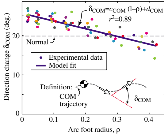
Fig. 5. The angular direction change \delta_{\text{COM}} in COM velocity decreased with increasing arc foot radius \rho . COM direction change was estimated as the angle between the steepest upward and downward velocities of the COM in the sagittal plane (defined below; compare with Fig. 1B). The relationship between \delta_{\text{COM}} and \rho is described well by the linear fit of Eqn 9, r^2=0.89 . Different coloured symbols indicate different subjects.
