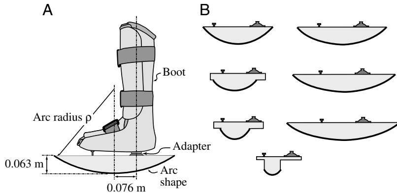
Fig. 3. Apparatus used to rigidly restrict human ankle motion and control rolling characteristics of the foot. (A) Subjects wore a boot and arc apparatus bilaterally, each consisting of a rigid walking boot modified to accept wooden arc shapes of varying radius. (B) 'Arc foot' shapes of varying arc radius \rho (defined as fraction of leg length) were rigidly attached with pyramidal prosthesis adapters. Arcs ranged in radius 0.02–0.40 m in absolute dimensions, and each subtended a sufficient range of angles to ensure continuous rolling ground contact throughout the stance phase. Arcs had matched mass of 1.1 \pm 0.1 kg, and boots had mass 0.85 or 1.05 kg, depending on size.
