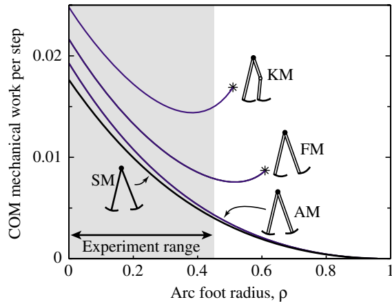
Fig. 2. Work performed on COM as a function of foot radius of curvature \rho , from various dynamic walking models. Models are powered by push-off to walk on level ground: the 'Simplest Model' (SM) with point mass pelvis and feet (Kuo, 2001), the 'Anthropomorphic Model' (AM) with human-like mass distribution (Kuo, 2001), the 'Forward-foot Model' (FM) with feet facing forward from the legs, and the 'Kneed Model' (KM) with knees and forward feet (after McGeer, 1990b). All simulations generally predict decreasing step-to-step transitions with increasing arc foot radius, roughly in proportion to (1-\rho)^2 as in Eqn 7. However, FM and KM have a slight upward trend for larger values of \rho , due to different foot geometry and introduction of knees. The SM is used as a prediction for experimental results. Over the range of arc radii studied experimentally, all other models match the trend of Eqn 7 reasonably well, with r^2 ranging 0.940–0.998.
