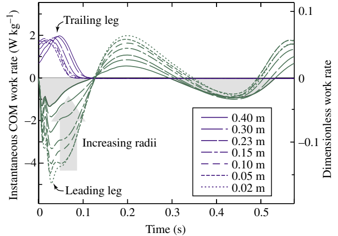
Fig. 6. Instantaneous COM mechanical work rate for each leg over one complete step, measured with arcs of different radii. The trailing leg performed positive work and the leading leg negative work to redirect the COM during the step-to-step transition. Leading leg negative work rate was highest in magnitude for small-radius arcs. Work rate magnitudes decreased with increasing arc radius for the leading leg during double support, and through most of single support. Average rate of negative work was computed by integrating the magnitude of negative regions of instantaneous work rate (shaded areas for 0.40 m arc) and dividing by step period. Data shown are averaged from all subjects and plotted over the mean step period. Blue and green traces indicate work rate of the trailing and leading leg, respectively.
