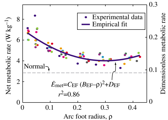
Fig. 8. Net metabolic rate \dot{E}_{\text{met}} exhibited a U-shaped curve as a function of arc radius \rho . For small radii, metabolic rate decreased with \rho much as predicted by the Simplest Model (Fig. 2). However, metabolic rate reached a minimum at \rho=0.30 according to the Empirical Fit of Eqn 11, r^2=0.86 , and began to increase with larger \rho . The energetic cost of walking was 59% higher than the minimum for the smallest arcs, and higher for all arc radii compared to normal walking (broken line). Different coloured symbols indicate different subjects.
