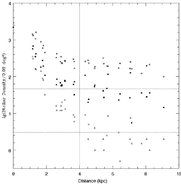
Fig. 16. Stellar density profiles of the C-type (triangles) and M-type (squares) AGB and RGB (stars) sources in each region in the multi-resolution grid (Fig. 15). The stellar density has been normalised to account for the varying area of each grid region. The horizontal lines at 1.66 and 0.48 represent the level of the remaining foreground contamination in the M- and C-type samples respectively. The vertical line at 4 kpc marks the limit of the detectable stellar component of NGC 6822.
