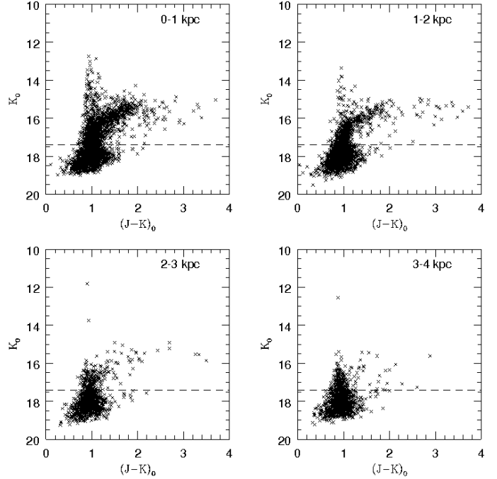
Fig. 24. CMD of the sources contained in each of the 4 annuli described in Sect. 4.4. The horizontal line in each frame marks the position of the TRGB at K_0 = 17.41 mag. No statistical adjustments have been made so foreground contamination that remained after the application of the J - H colour selection is also present in the CMDs and is expected to become increasingly significant with increasing radial distance. The total number of sources and the total number of AGB sources is 2683 and 1325 respectively in the 0–1 kpc annuli, 1823 and 580 in the 1–2 kpc annuli, 1052 and 230 in the 2–3 kpc annuli and 1115 and 233 in the 3–4 kpc annuli.
