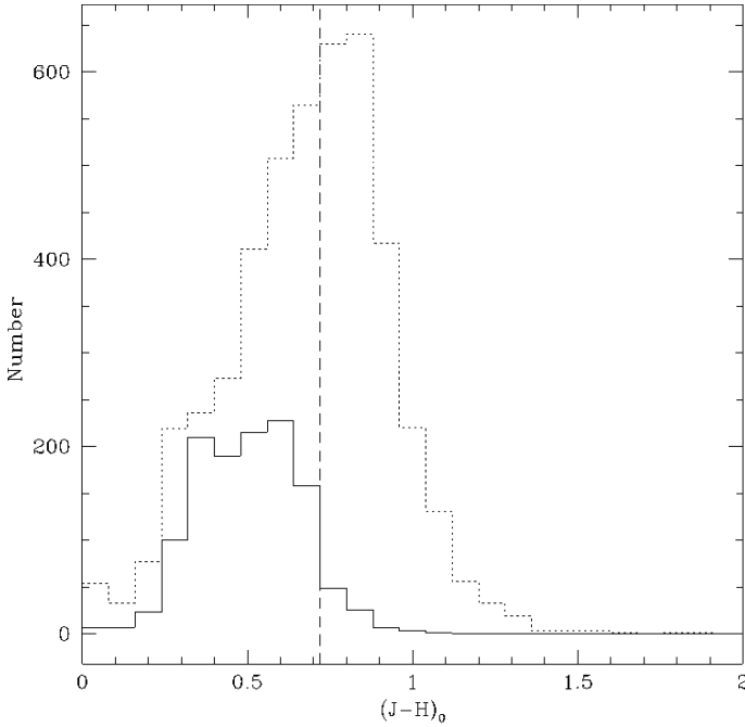
Fig. 7. Colour histograms with bin size 0.1 mag, of the same sources as in Fig. 6. The dotted-line histogram corresponds to the central region of the galaxy and the solid-line histogram corresponds to the outer region. The dashed vertical line is at (J - H)_0 = 0.72 mag.
