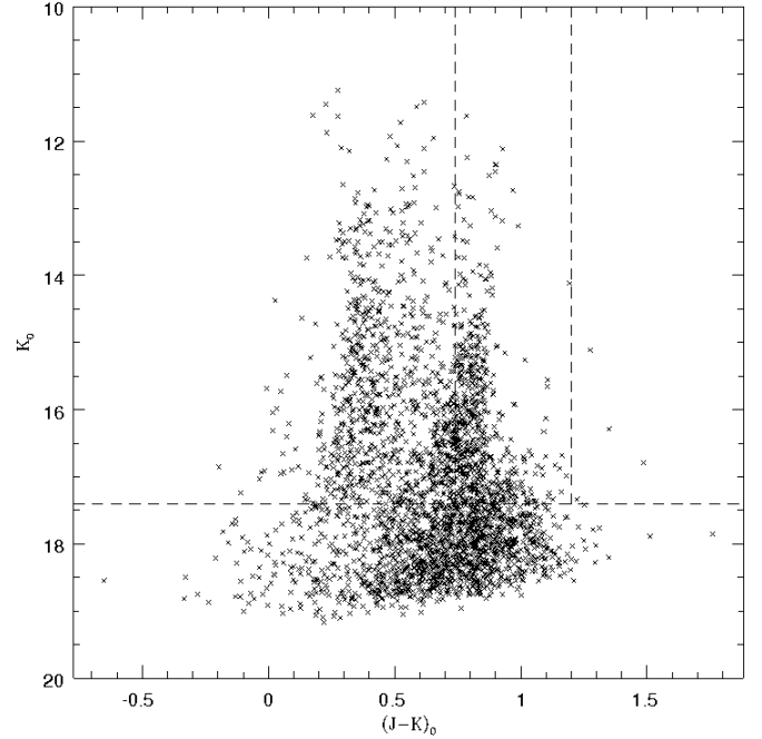
Fig. 13. CMD of the MW sources located in the over-density in the centre of Fig. 12. The horizontal and vertical lines represent the position of the TRGB and the colour selection criteria for the selection of C- and M-type AGB stars, respectively, as in Fig. 8.
