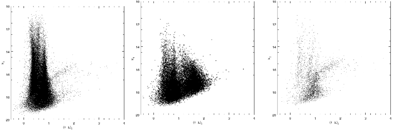
Fig. 4. Left: CMD of all the stellar and probably-stellar sources, including Milky Way foreground and genuine NGC 6822 stars. Middle: CMD of the non-stellar sources from the original photometric catalogue in the direction of NGC 6822. Right: CMD of the stellar and probably-stellar sources from the centre of the observed area – MW foreground contamination is still present but the CMD is dominated by sources belonging to NGC 6822. The peak belonging to the M-type stars and the diagonal branch generated by the C-type stars are more easily distinguished here.
