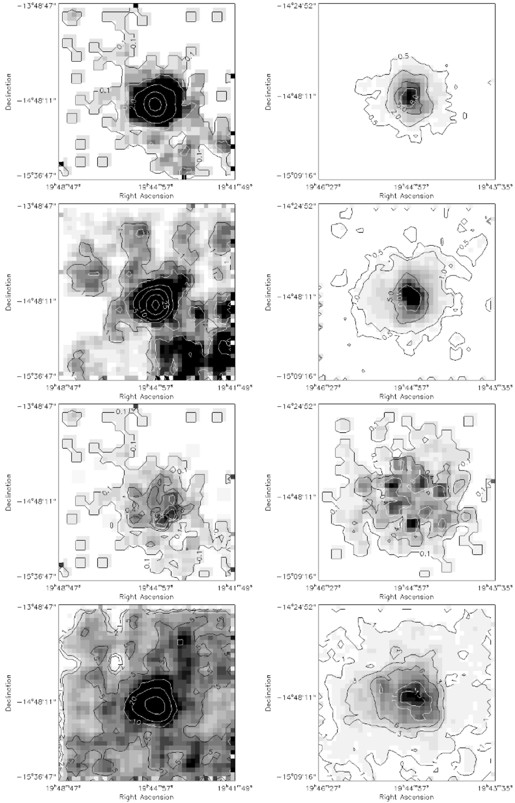
Fig. 11. From top to bottom, density distribution of: carbon-rich stars, oxygen-rich stars, the C/M ratio and RGB stars. Each row shows, on the left a map of the full observed area using 1600 bins and on the right a map of the central 34' \times 34' also using 1600 bins. Contours are at: 0.1, 0.5, 2, 10 and 15 for carbon-rich stars in low resolution map and 0.5, 2, 5 and 8 in the high resolution map. For oxygen-rich stars contours are at: 1, 2, 5, 10, 25 and 50 in the low resolution map and 0.5, 1, 5 and 10 in the high resolution map. For the C/M ratio the contours are at: 0.1, 0.4, 0.6, 0.8 and 1 in the low resolution and 0.1, 0.4 and 0.8 in the high resolution map. For the RGB stars contours are at: 1, 2, 5, 10, 20 and 50 in the low resolution map and at 1, 3, 6, 11 and 15 in the high resolution map. At a distance of 490 kpc, the full field is 14.5 \times 14.5 \text{ kpc}^2 , whilst the high resolution field is 4.85 \times 4.85 \text{ kpc}^2 .
