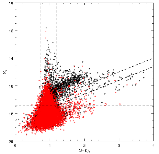
Fig. 17. CMD of all the remaining sources after the removal of the foreground (black) and only those sources belonging to the medium and coarse grid regions (red) in Fig. 15. The horizontal line represents the position of the TRGB at K_0 = 17.41 mag. The vertical lines represent the colour selection criteria at (J - K)_0 = 0.74 and 1.20 mag. The diagonal lines at J_0 = 18.61 and 18.0 mag represent alternative selection criteria (see Sect. 5.3.3).
