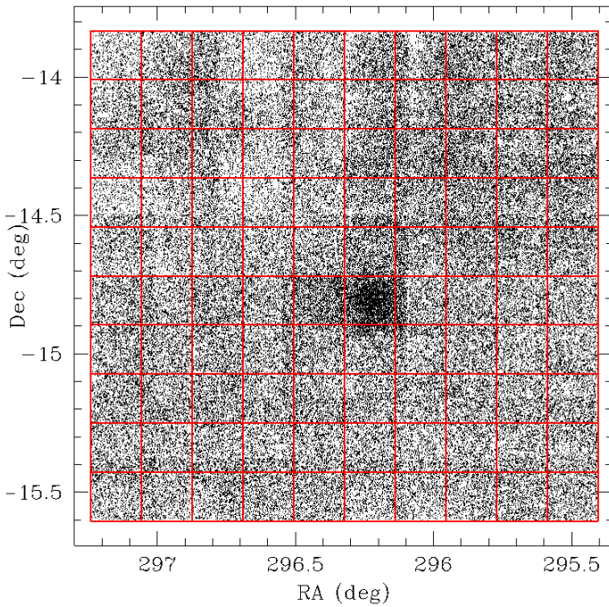
Fig. 5. The division of the observed area into a grid of 100 regions, each of dimensions 10' \times 10' , prior to foreground removal. The sources shown have been defined as stellar or probably-stellar in all three photometric bands, no other selection criteria have been applied. Some of the patchiness seen here is the result of varying limiting magnitudes in the observations – particularly in the NE footprint.
