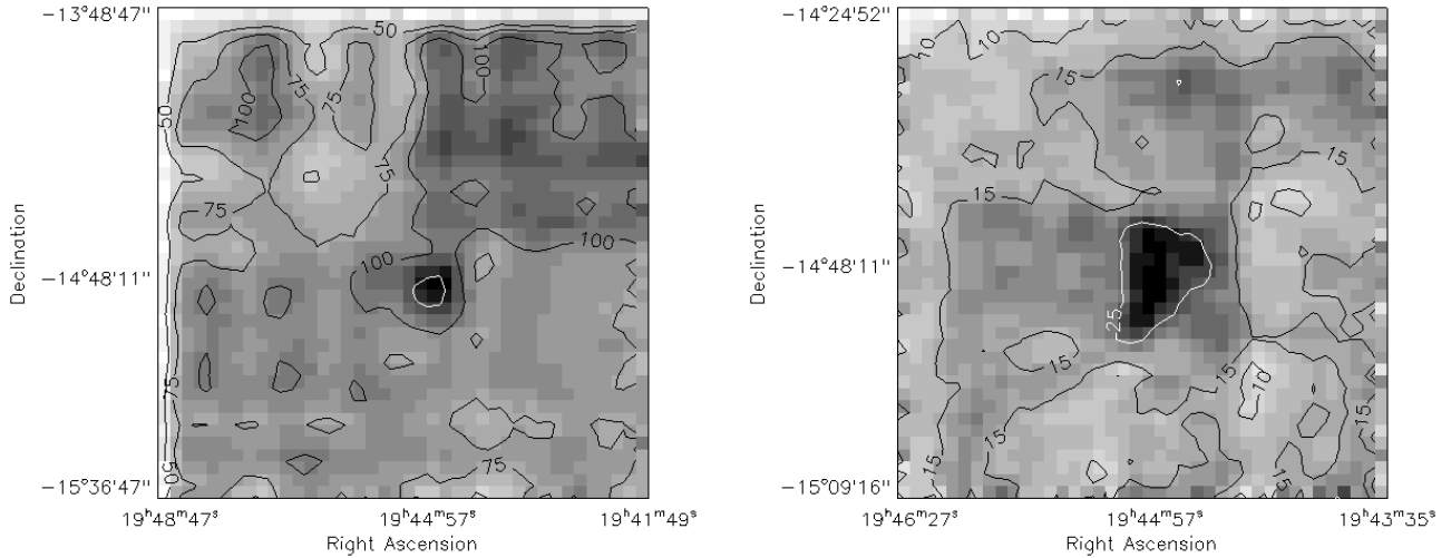
Fig. 12. Density distribution of foreground sources removed from the data set as described in the text. On the left using 1600 bins across the full observed area contours are at 50, 75, 100 and 150. On the right is the high resolution plot, contours are at 10, 15 and 25.
