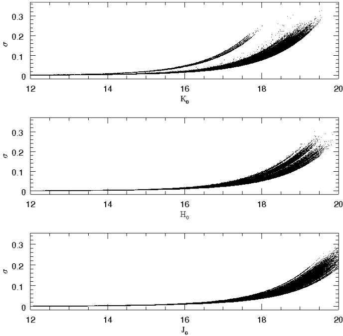
Fig. 2. Magnitude vs. error for each photometric band. The branch that splits away from the main body of sources at \sim 15 mag in the K -band shows the increased error associated with the subset of data from the NE region that was collected during a technical fault.
