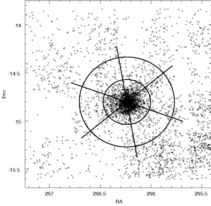
Fig. 18. To study variations in the TRGB magnitude, C/M ratio and [Fe/H] as a function of azimuthal angle the region inside 4 kpc has been divided into 12 regions – 2 annuli between 0–2 kpc and 2–4 kpc with each annuli further divided into 6 regions at intervals of 60°.
