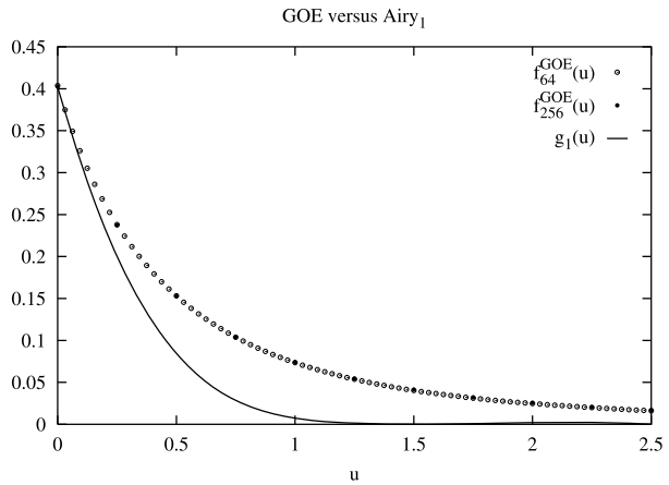
Fig. 1 The covariance g_1 of the Airy 1 process (line) versus the one of the largest eigenvalue for GOE matrix diffusion, f_N^{\text{GOE}} , for N = 64, 256
