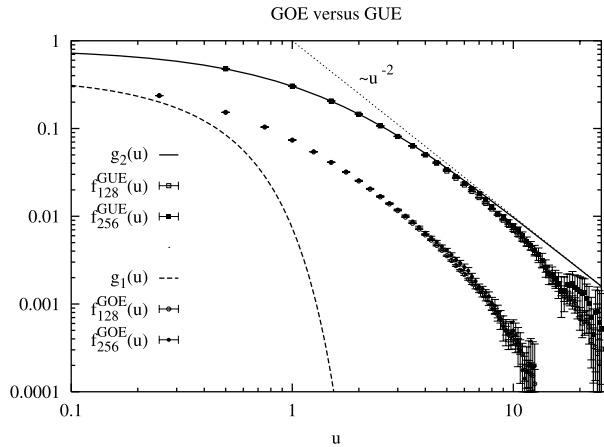
Fig. 3 Log-log plot of the rescaled correlation functions for GOE and GUE
