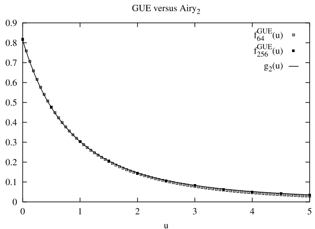
Fig. 2 The covariance g_2 of the Airy 2 process (line) versus the one of the largest eigenvalue for GUE matrix diffusion, f_N^{\text{GUE}} , for N = 64, 256
