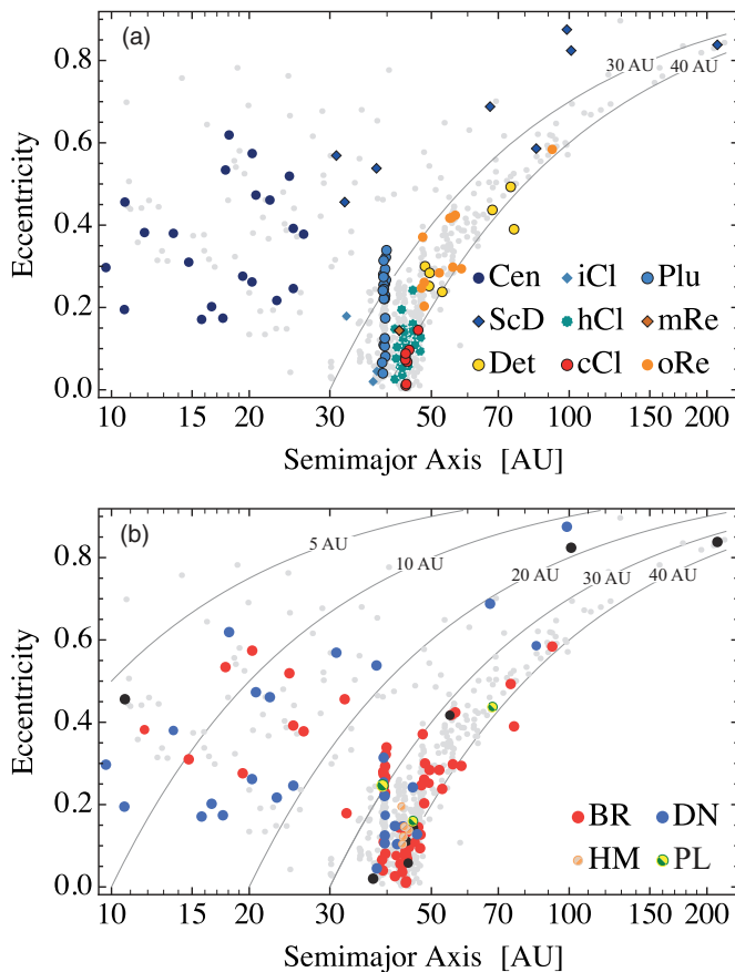
Figure 1. (a) Orbital distribution (semimajor axis vs. eccentricity) of our sample (Cen = Centaurs, iCl = inner classical, Plu = Plutinos, ScD = scattered disk, hCl = hot classical, mRe = middle resonant, Det = detached, cCl = cold classical, oRe = outer resonant). The light gray points mark TNOs not observed by Herschel . The curves of constant perihelion are plotted in solid gray and labeled. (b) Same as panel (a), but color-coded by surface type (BR = bright red, DN = dark neutral, HM = Haumea-type, PL = dwarf planet, black points have large uncertainties and ambiguous surface type.)
