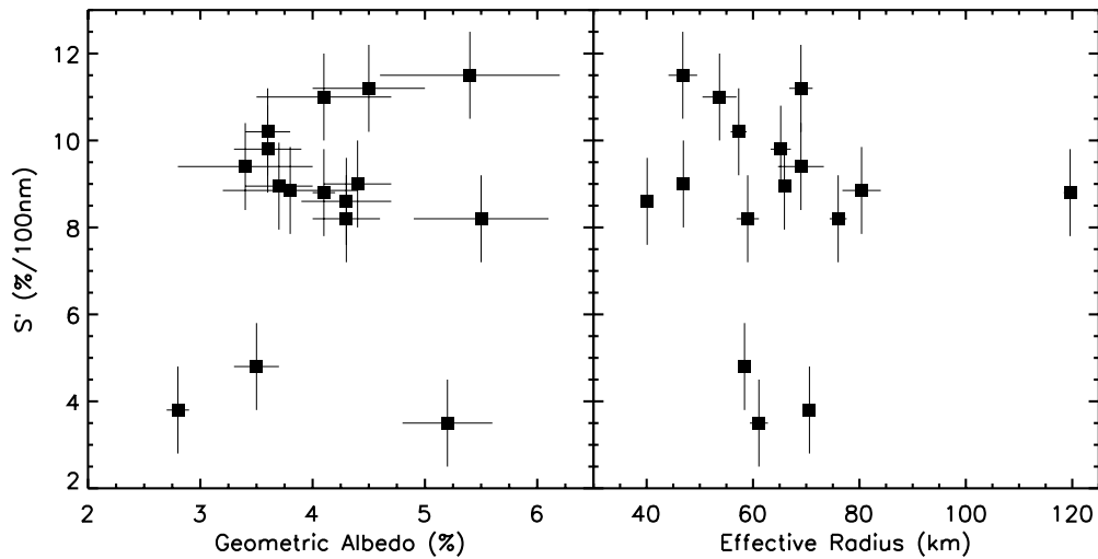
FIG. 3.—Comparison between our measured albedos and effective radii and the visible-wavelength spectral slopes reported by Jewitt & Luu (1990) and Fitzsimmons et al. (1994). We have used the results from the \eta = 0.94 case here. The ordinate is S' , the percentage change in reflectance per 100 nm, as reported by those authors. As in Fig. 2, there is only a weak correlation in each plot.
