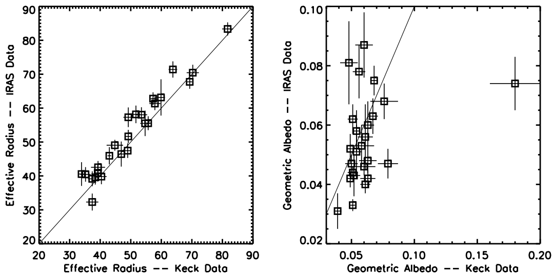
FIG. 4.—Comparison of our radiometric radii and albedos with those found by Tedesco et al. (2002) from IRAS data for objects common to both surveys. Since IRAS results employed \eta = 0.756 , we have used our results from that case as well. Diagonal lines indicate the equivalence of the two measurements. The radii are very similar, indicating that the MIR data are robust, but there is wide variation in the albedos. This shows the importance of having complementary visible-wavelength data, as in the present work.
