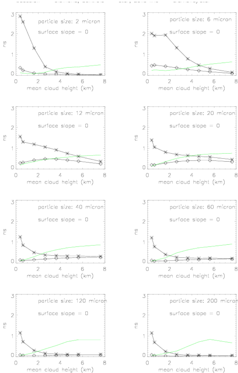
Figure 10 - Bias in ns from Surface Elevation; Star - Centroid of the Return, Diamond - Centroid of the Gaussian Fit
