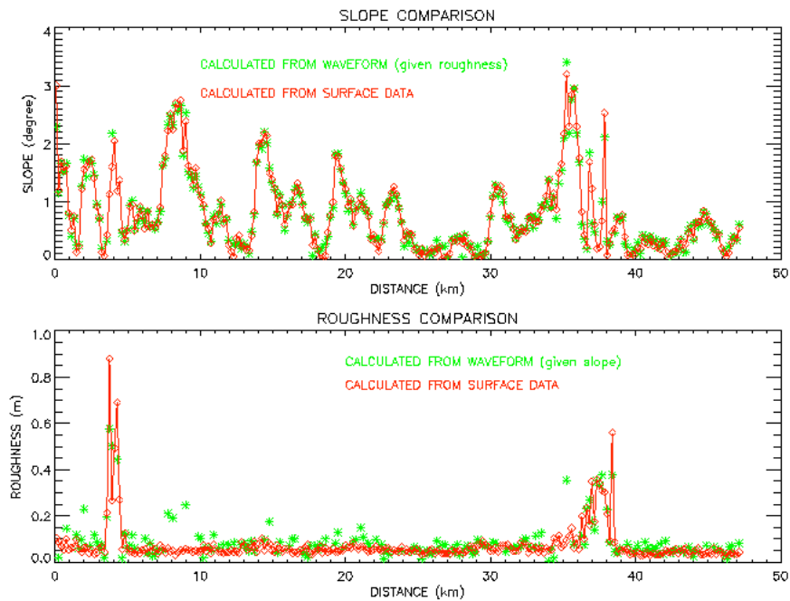
Figure 12 - Comparison of Actual vs Calculated Surface Roughness and Slope (no longer calculated).
