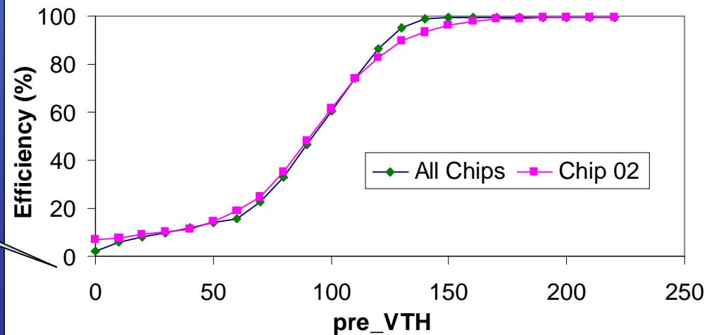
Threshold scan (LADDER-Chip02)
