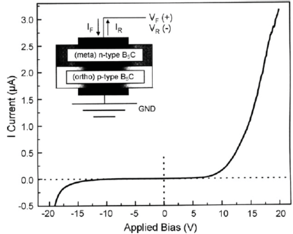
Figure 4. The I(V) characteristic curve of a 2 \mu\text{m} thick p-type boron carbide semiconducting polytype to n-type boron carbide semiconducting polytype diode at 295 K, as described in [4], and in the text. The inset is a schematic of the diode construction.
