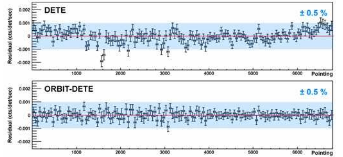
Fig. 3. Residual count rate as function of pointing number for the DETE (top) and ORBIT-DETE (bottom) background models for the energy band 507.5–514.5 keV. In addition to the background models the best fitting 2d Gaussian surface brightness model (cf. Sect. 4.2.2) has been subtracted from the data. For clarity, the data have been rebinned into groups of 50 pointings. The shaded area indicates count rate variations of \pm 0.5\% . For comparison, the maximum 511 keV line signal amplitude corresponds to approximately \sim 2\% of the observed count rate.
