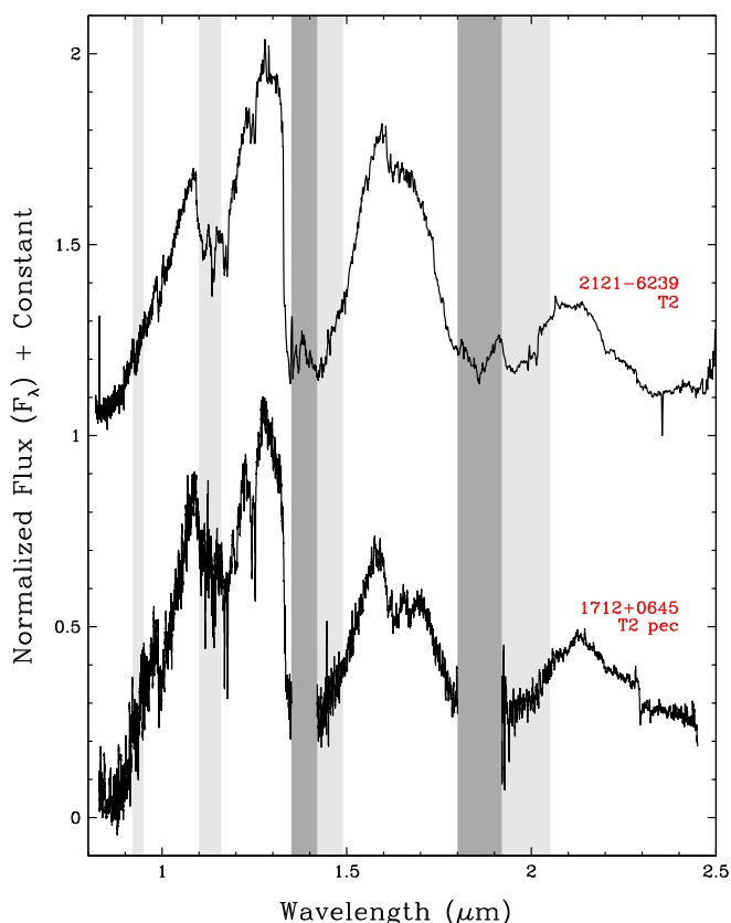
Figure 55. Spectra of T dwarfs. (See the caption of Figure 52 for other details.)
