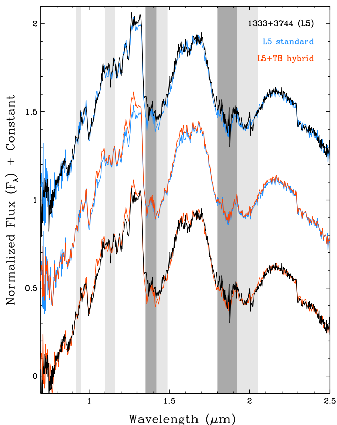
Figure 54. Comparison of the best fitting standard, the L5 (top), and the best fitting synthetic binary, the L5+T8 (bottom), to the spectrum of WISE 1333+3744. (See the caption of Figure 52 for other details.)
