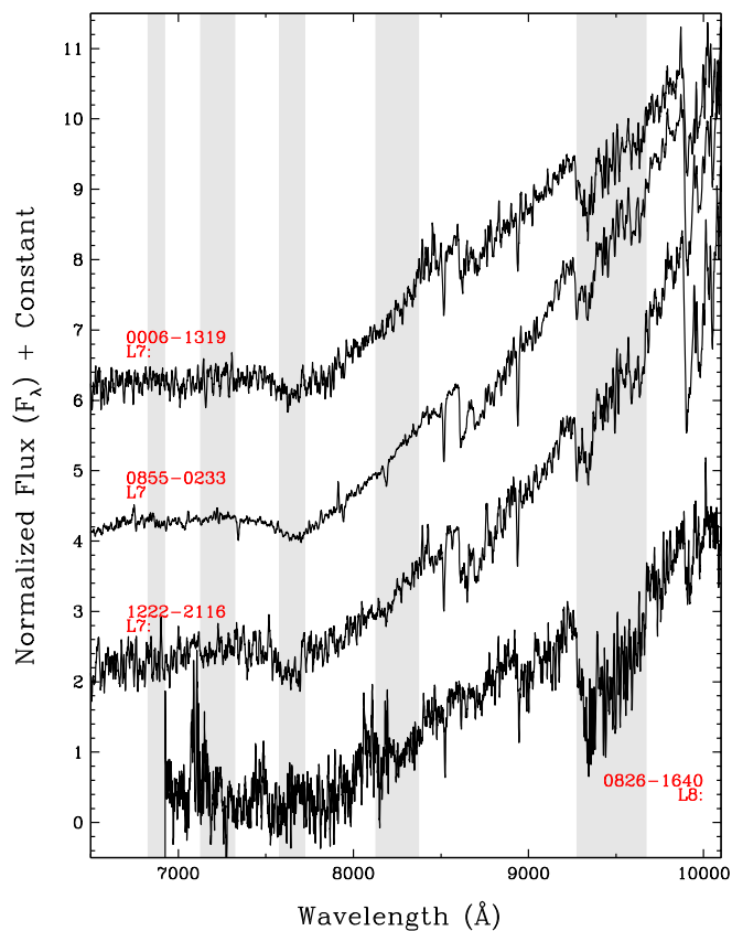
Figure 51. Spectra of dwarfs with types of L7 through L8. (See the caption of Figure 48 for other details.)
