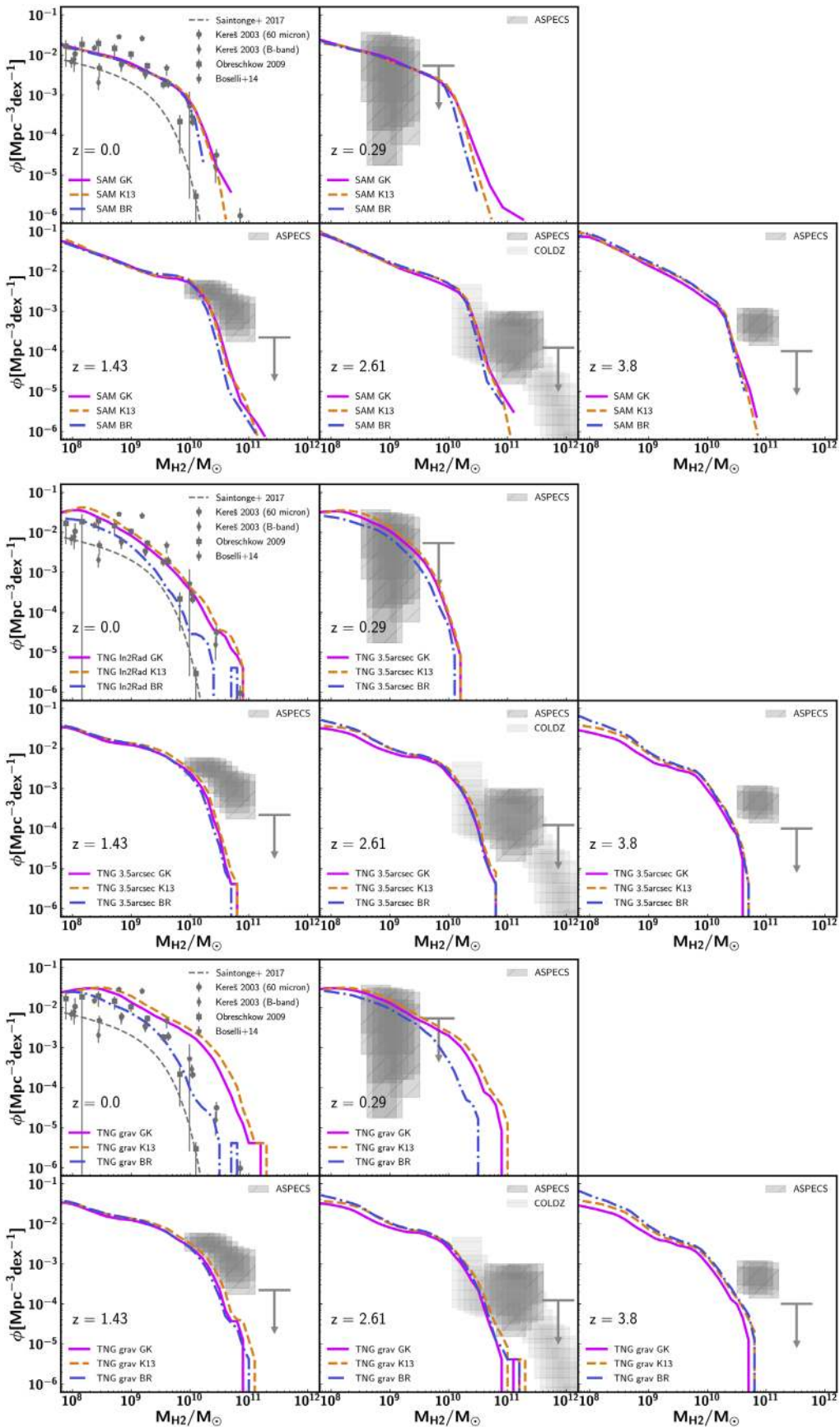
Figure 9. H_2 mass function of galaxies at z = 0 and the redshifts probed by ASPECS. Model predictions are shown for the SC SAM (top two rows), IllustrisTNG adopting the “3//5” aperture (middle two rows, note that at z = 0 this is replaced by then “In2Rad” aperture) and IllustrisTNG when adopting the “Grav” aperture (bottom two rows). For all models we show the GK (solid pink), the K13 (dashed orange), and the BR (dashed–dotted blue) H_2 partitioning recipes. The data comparison is identical to that of Figure 3.
