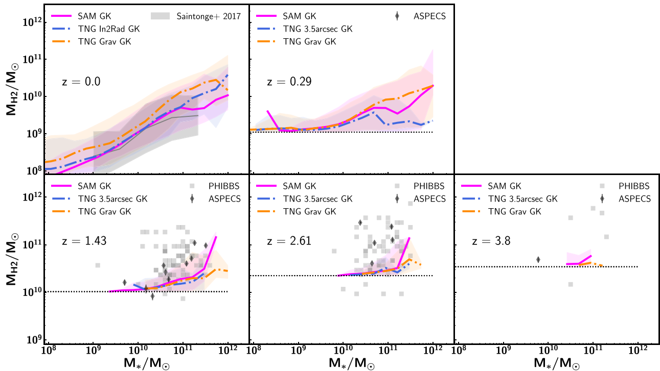
Figure 2. Predicted and observed H_2 mass of galaxies at different redshifts as a function of their stellar mass. For the theoretical data, we account for observational selection effects. The results from SC SAM (solid pink) and from IllustrisTNG are shown by adopting the GK H_2 partitioning recipe. We show predictions for IllustrisTNG when adopting the “3//5” (dashed blue) and “Grav” (dotted–dashed orange) apertures (at z = 0 , the “3//5” aperture is replaced by the “In2Rad” aperture). In this figure we assume \alpha_{CO} = 3.6 M_\odot / (\text{K km s}^{-1} \text{pc}^2) . At z = 0 a comparison is done to observational data from Saintonge et al. (2017). To allow for a fair comparison and remove the contribution by quiescent galaxies, a selection criterion of \log \text{SFR} > \log \text{SFR}_{\text{MS}}(M_*) - 0.4 is applied to both the observed and modeled galaxies at z = 0 , where \log \text{SFR}_{\text{MS}}(M_*) marks the SFR of galaxies on the main sequence of star formation, following the definition of Speagle et al. (2014). At higher redshifts model predictions are compared to the detections of ASPECS, as well as the compilation of CO detected galaxies presented as a part of PHIBBS in Tacconi et al. (2018). At these redshifts the ASPECS selection function is applied to the model galaxies (and depicted by the dotted black horizontal line). The solid lines mark the median of the galaxy population, whereas the shaded regions mark the 2\sigma scatter of the population. The different models are only partially able to reproduce the ASPECS and PHIBBS detections. We furthermore find that the ASPECS sensitivity sets a strong cut on the overall galaxy population (compare to Figure 1).
