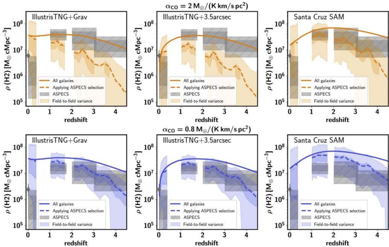
Figure 7. Model predictions for the \text{H}_2 cosmic density as a function of redshift as predicted from IllustrisTNG adopting the “Grav” aperture (left), IllustrisTNG adopting the “3//5” aperture (middle), and the SC SAM (right column), all of them adopting the GK \text{H}_2 partitioning recipe. The first and second rows correspond to a scenario where we adopt a CO-to- \text{H}_2 conversion factor of \alpha_{\text{CO}} = 2.0 M_{\odot}/(\text{K km s}^{-1} \text{pc}^2) and \alpha_{\text{CO}} = 0.8 M_{\odot}/(\text{K km s}^{-1} \text{pc}^2) for the observations, respectively. The solid lines correspond to the cosmic \text{H}_2 density based on all the galaxies in the simulated volume, ignoring any selection function. The dashed lines correspond to the cosmic \text{H}_2 density in the entire box, applying the ASPECS selection function. The shaded regions mark the 2\sigma and 1\sigma scatter when calculating the \text{H}_2 mass function in 1000 randomly selected cones that capture a volume corresponding to the volume probed by ASPECS at the given redshifts, also applying the ASPECS selection function. Model predictions are compared to the observational results from ASPECS (dark (light) gray mark the 1\sigma ( 2\sigma ) uncertainty), as well as observations at z = 0 from Keres et al. (2003) and Obreschkow & Rawlings (2009).
