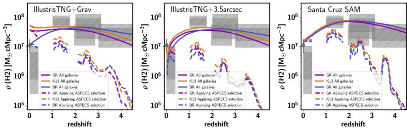
Figure 10. Model predictions for the H_2 cosmic density as a function of redshift as predicted from IllustrisTNG when adopting the “Grav” aperture (left), IllustrisTNG when adopting the “3/5” aperture (middle), and the SC SAM (right). We show the the GK (pink), K13 (orange), and BR (blue) H_2 partitioning recipes for all models. The solid lines correspond to the cosmic H_2 density in the entire box, ignoring any selection function. The dashed lines correspond to the cosmic H_2 density in the entire box, applying the ASPECS selection function. Model predictions are compared to the observations from ASPECS (dark (light) gray mark the 1\sigma ( 2\sigma ) uncertainty), as well as observations at z = 0 from Keres et al. (2003) and Obreschkow & Rawlings (2009).
