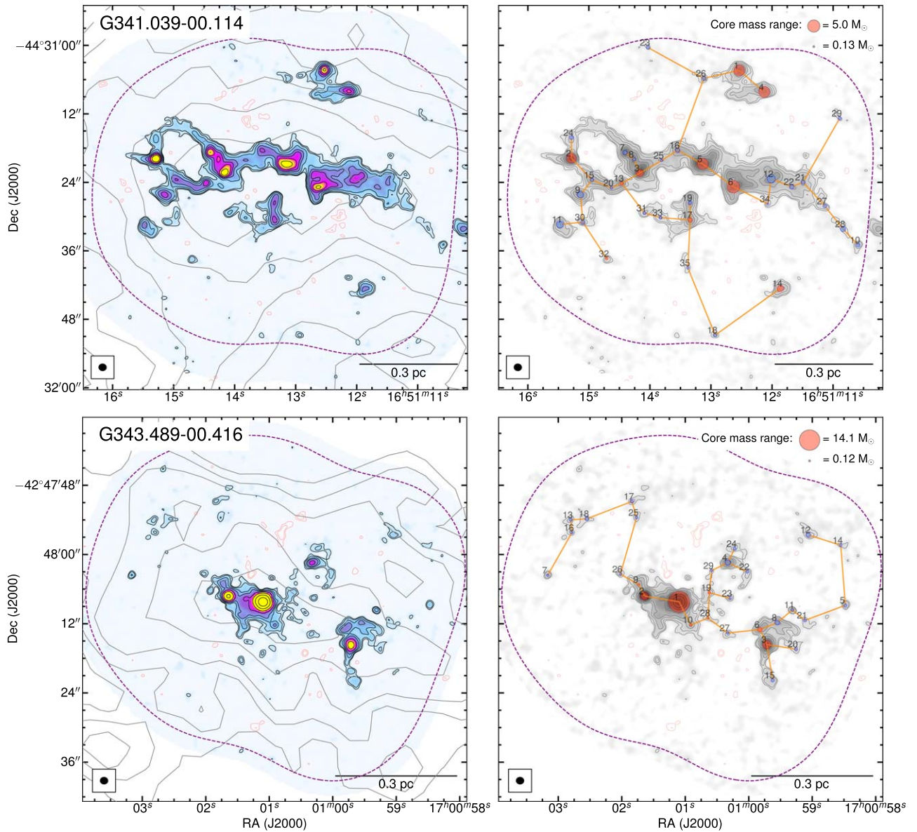
Figure 10. Same as in Figure 5, except for ALMA contour levels of -4, -3, 3, 4, 6, 9, 12, 16, and 22 \times \sigma , with \sigma = 0.070 mJy beam ^{-1} , for G341.039–00.114 ( 1''.2 angular resolution); and -4, -3, 3, 4, 6, 8, 12, 20, 40, and 100 \times \sigma , with \sigma = 0.068 mJy beam ^{-1} , for G343.489–00.416 ( 1''.2 angular resolution).
