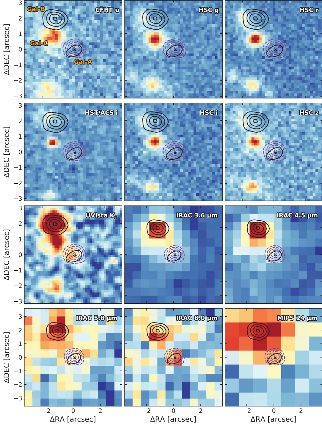
Figure 3. Cutouts centred on Gal–A in different photometric filters, from HST/ACS (Koekemoer et al. 2007) and Subaru , UltraVISTA, and Spitzer (Capak et al. 2007; Laigle et al. 2016). The violet dashed and black solid contours are >3\sigma line and continuum emissions (at steps of 2\sigma ), respectively. Gal–A, Gal–B, and Gal–C are labelled in the upper left plot of the figure. Wavelengths increase from the upper left to the bottom-right corner.
