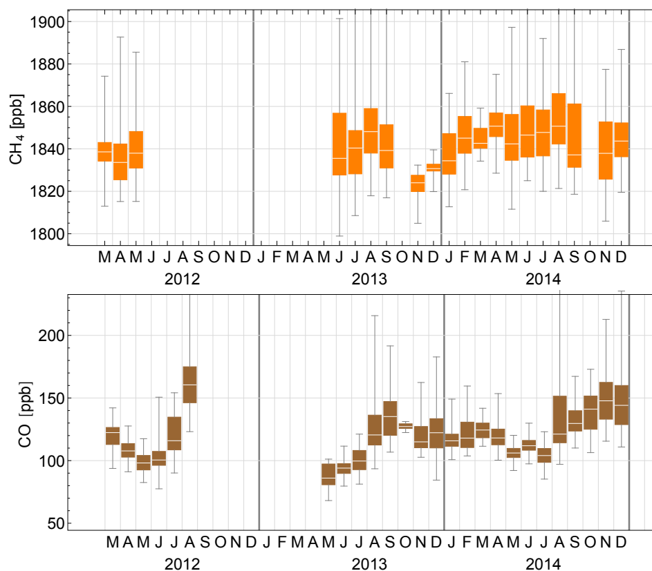
Figure 20. Statistics of monthly daytime (17:00–20:00 UT) 30 min measurements of \text{CH}_4 and CO at the 79 m level of the 80 m walk-up tower. Shown are whisker plots indicating min/max and quartiles of the monthly measurements. The white line in the box indicates the median.
