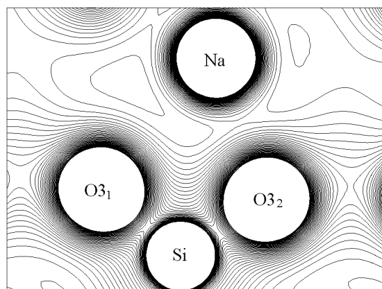
FIGURE 2. An example of interactive displays that can be created by the software associated with the American Mineralogist Crystal Structure Database. The example includes images of (a) the crystal structure of jadeite in a combined polyhedral and ellipsoidal rendering made with XtalDraw; (b) the powder diffraction pattern of jadeite using MoK \alpha radiation made with XPOW; and (c) an electron density map of the plane through Na and bridging O atoms in jadeite made with SPEEDEN.
