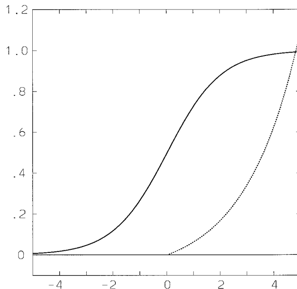
FIG. 8. Two possible nonlinear filter functions that relate the input and output of a neuron in a neural net. Bold line is a classical sigmoidal type; the dashed line represents Eq. (12), more suitable for the simulation of daily rainfall. In this plot x_c = 0 .
