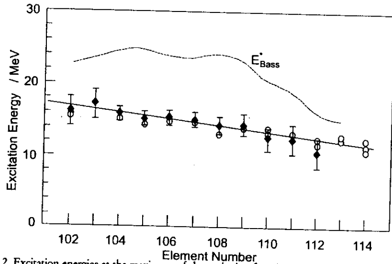
Fig. 2. Excitation energies at the maximum of the excitation functions of (HI, 1n) reactions leads to nuclei with Z=102-114 , o -- theoretical (see Table I) and black signs - experimental data [8].
