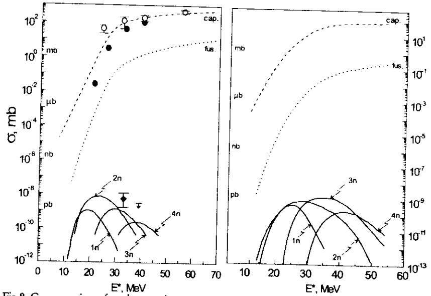
Fig.8 Cross sections for the reactions ^{48}\text{Ca}+^{238}\text{U} (left) and ^{48}\text{Ca}+^{244}\text{Pu} (right) leading to compound nuclei with Z=112 and Z=114 , respectively. On the left, open and solid circles are capture cross sections from Ref.[25] and [26] correspondingly. Experimental data for \sigma_{xn} was taken from [27]. Different curves are theoretical calculations (explanation see in the caption of Fig.7).
