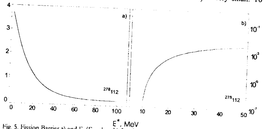
Fig. 5. Fission Barrier a) and \Gamma_n/\Gamma_f values b) for element 112 as a function of excitation energy.
