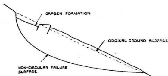
Fig. 1. Graben formation due to non-rotational slip
