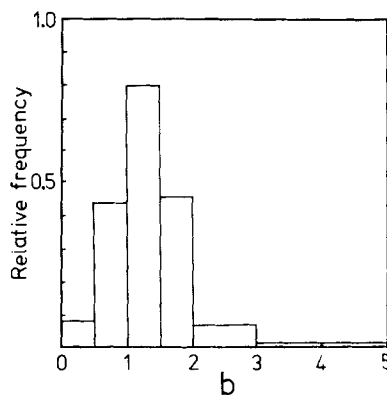
Figure 1. Frequency distribution of b for overcast hours. The frequencies are expressed per unit range of b to allow for unequal ranges.
