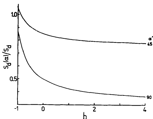
Figure 2. The relative irradiance S_d(\alpha)/S_d of planes with slope \alpha = 45^\circ and 90^\circ as a function of the parameter b .
