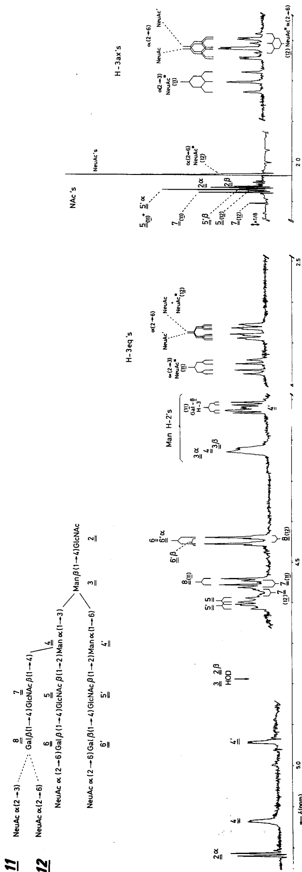
Fig. 12. Structural reporter group regions of the resolution enhanced 500-MHz ^1\text{H-NMR} spectrum of a mixture of trisialo compounds 11 and 12 , differing in the type of linkage of NeuAc* to Gal-8, in ratio 92:8, together with the structures. The double-underlined numbers in the spectrum refer to the corresponding residues in the structures. Signals stemming from corresponding protons of compounds 11 and 12 coincide, unless otherwise indicated (see Table 4). The relative intensity scale of the N -acetyl proton region differs from that of the other parts of the spectrum as indicated. The HOD-resonance, as well as the H-1 signals of Man-3 and GlcNAc-2 ( \beta ) which at a sample temperature of 300 K are partially hidden under this line, are left out from the spectrum; the position of the HOD-line is indicated by an arrow.
