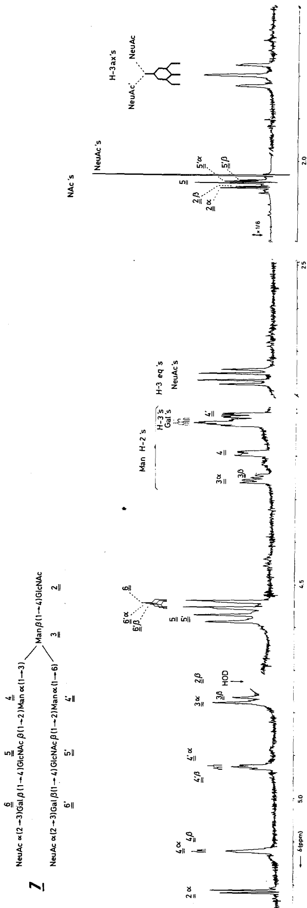
Fig. 8. Structural reporter regions of the resolution enhanced 500-MHz 1 H-NMR spectrum of compound 7, together with its structure. The numbers in the spectrum refer to the corresponding residues in the structure. The relative intensity scale of the N -acetyl proton region differs from that of the other parts of the spectrum as indicated. The HOD-resonance and the H-1 doublet of the β-anomer of GlcNAc-2, almost coinciding at a sample temperature of 300 K, are left out from the spectrum; their rough position is indicated by an arrow.
