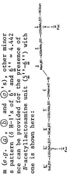
Fig. 14. Structural reporter group regions of the resolution enhanced 500-MHz 1 H-NMR spectrum of a mixture of 14 , 15 , the bifuco mono-antennary glycopeptides 14 , 15 and 16 , in ratio 6:1:1, together with their structures. The double-underlined numbers in the spectrum refer to the corresponding residues in the structures. Signals stemming from corresponding protons of compounds 14 , 15 and 16 coincide, unless otherwise indicated (see Table 5). The relative intensity of the N -acetyl proton region differs from that of the other parts of the spectrum as indicated. The HOD-resonance is left out from the spectrum; its position is indicated by an arrow. As is obvious from the presence of not yet assigned resonances in the spectrum ( e.g. 14 , 15 and 16 ), other minor components are present in this glycopeptide mixture. Mainly from the Gal H-1's pattern ( \delta H-1's of 14 ' and 16 ' = 4.442 and 4.456 ppm) as well as from the H-4 signal of Gal-6' at \delta \approx 4.18 ppm evidence can be provided for the presence of a mono-antennary lower branch glycopeptide, containing a so-called additional N -acetylglucosamine unit ( 15 '- 16 ') with Fuc \alpha(1-3) linked to GlcNAc- 5 ', in the mixture. The structure of the latter one is shown here:
