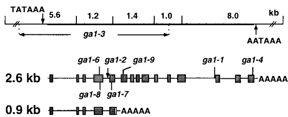
Figure 2. Physical Map of the GA1 Locus.
