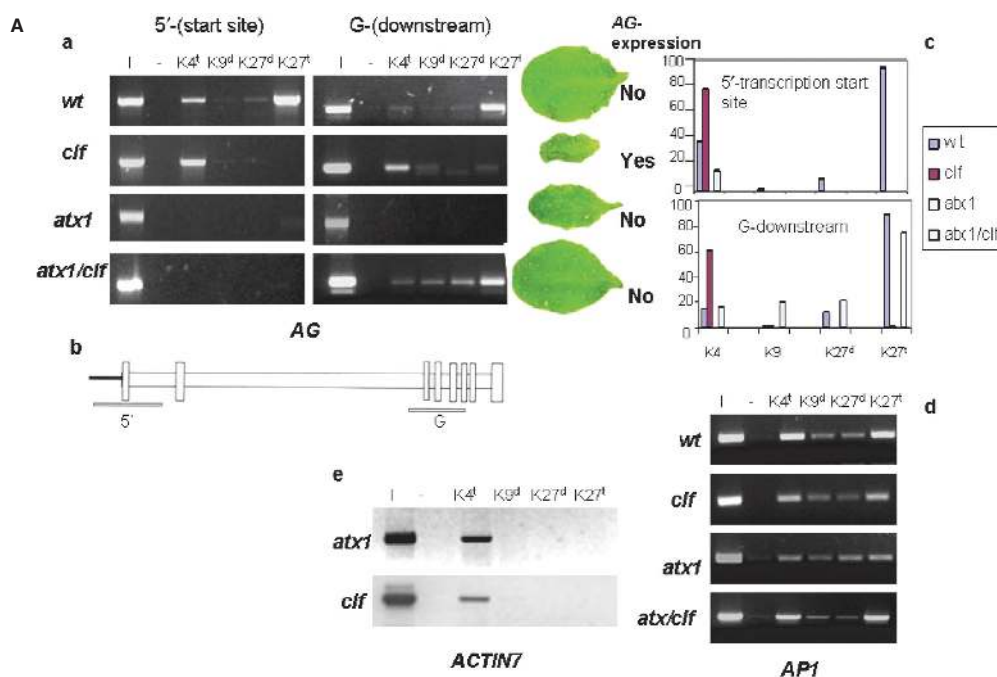
Figure 3. Methylation profiles of histone H3-tail lysines of AG -nucleosomes. (a) ChIP assays with antibodies specific against tri-methylated H3K4 and tri-methylated H3K27, and di-methylated H3K9. Amplified regions are from the 5'-transcription start site and from downstream gene (G)-regions (see b). The characteristic leaf phenotypes are shown in parallel with the methylation patterns at 5'-end and downstream nucleosomes, and corresponding expression of AG is indicated; (b) schematic representation of the AG gene: empty vertical boxes represent exons, horizontal boxes represent introns. Bars below the line show regions amplified in the PCR-assay; 5'-represents the region upstream of the transcription start site; G (gene) stands for downstream coding sequences; (c) quantified bands showing the relative change in methylation modifications at the 5'-end and the downstream (G)-nucleosomes; results are from three independently performed ChIP assays; (d) the API -methylation profiles are shown as controls illustrating the quality of the templates; the same amounts of template DNA were used in the respective amplification experiments and (e) ACTIN7 , a constitutively expressed gene carries only 'activating' m 3 K4/H3 tags.
