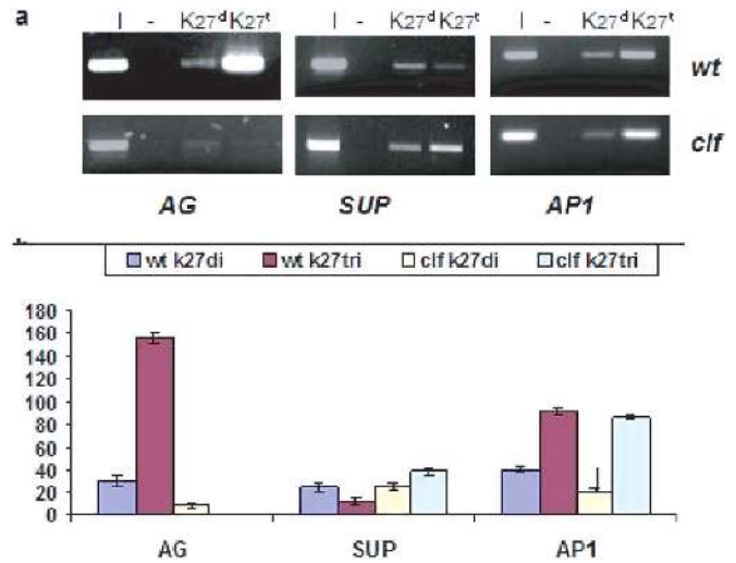
Figure 2. H3K27me2 and H3K27me3 profiles of three Arabidopsis genes. (a) ChIP assays with antibodies specific against di- and trimethylated H3K27; superscripts 't' and 'd' stand for the tri- or dimethylated isoforms, respectively. (I)-input sample is 15% of the immunoprecipitated DNA; (-) is negative control without antibody. Quantified bands from three independently performed ChIP assays are shown as graphs. Changes in H3K27me3 levels of wild type and clf SUP and API nucleosomes are insignificant ( p > 0.5 ).
