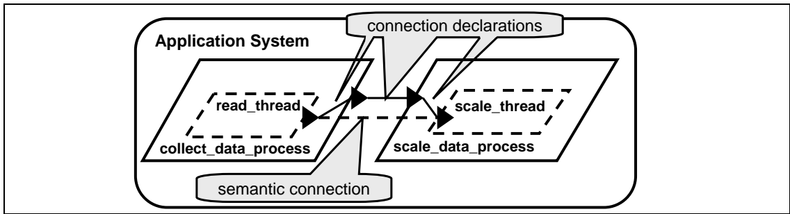
Figure 8-2: A Semantic Connection between Thread Instances
