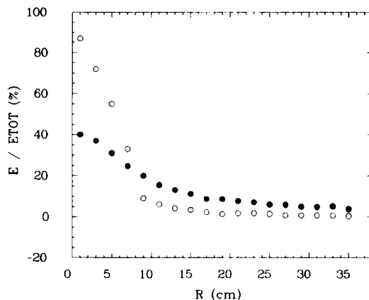
Fig. 10. Fraction of the total shower energy deposited in the distance R from the impact point for electrons (open circles) and hadrons (full circles) depositing E \geq 0.6 GeV in the calorimeter.
