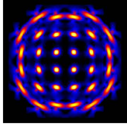
Fig. 14. ART-XC PSF model applicable to data of survey and scanning observations, for various source positions in the telescope field of view, at 8.1 keV.
