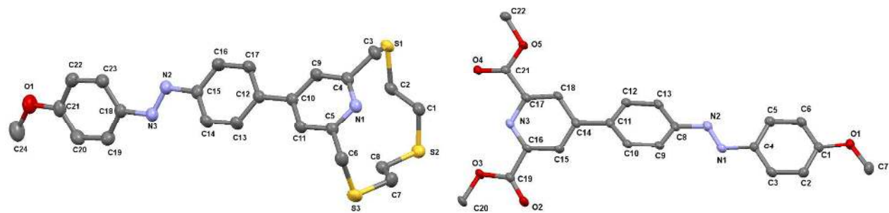
Figure 2: X-ray crystal structures of ligand 13 and azo-dye 14 (Ellipsoids at 50% probability level. Selected bond lengths and torsion angles are to be found in the ESI).
