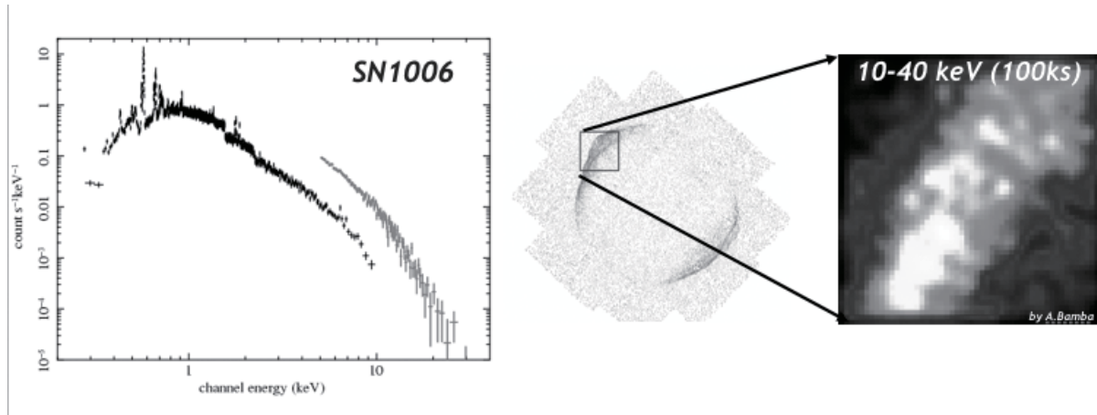
Figure 9. (left) Simulated spectra for 100 ks SXS observation of SN1006 with SXS and HXI. (right) Image expected from the combination of HXT and HXI.
