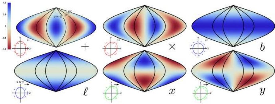
Fig. 12 The induced variations in the observed pulse phase as a function of pulsar sky location for a long-wavelength GW traveling along the positive z -axis. The scalar/vector/tensor and longitudinal/transverse nature of each polarization mode is apparent
